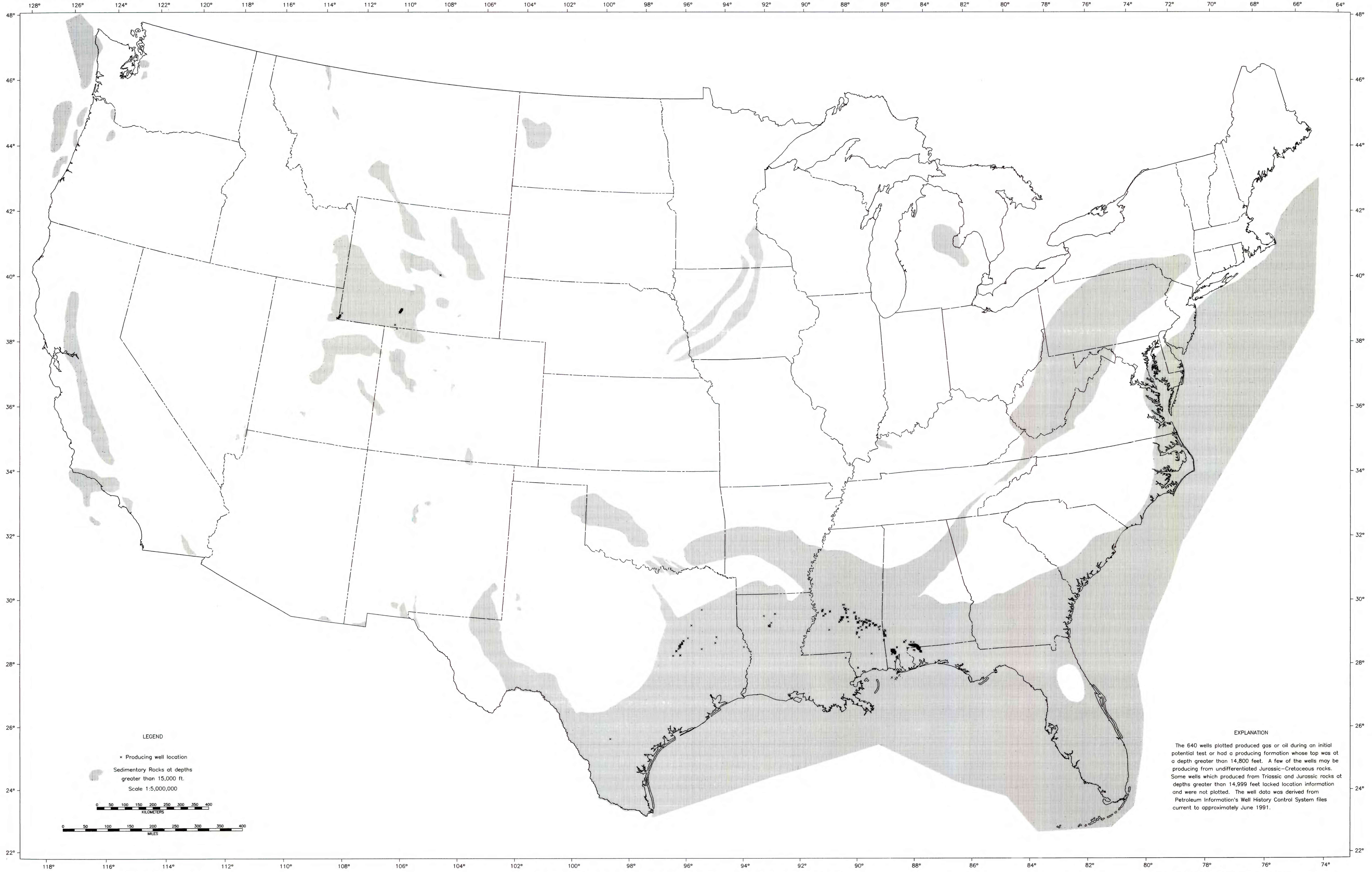
LOCATION OF WELLS IN THE UNITED STATES PRODUCING HYDROCARBONS FROM TRIASSIC AND JURASSIC ROCKS AT DEPTHS GREATER THAN 14,999 FEET
