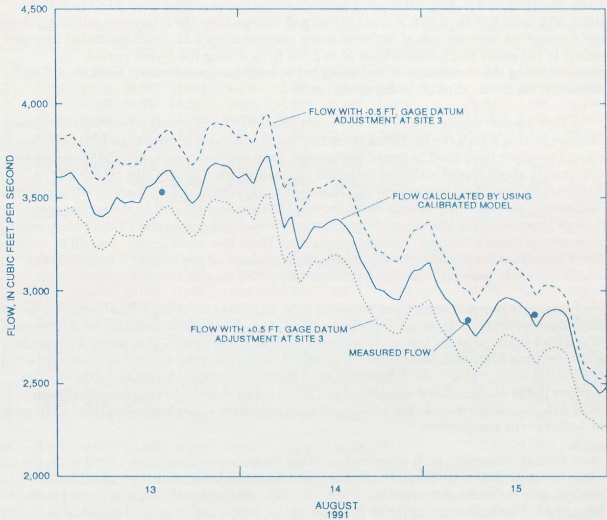
Figure 14.--Simulated flow in the Roanoke River at site 3 for the period August 13-15, 1991, using calibrated model, gage datum increased by 0.5 foot, and gage datum reduced by 0.5 foot.
