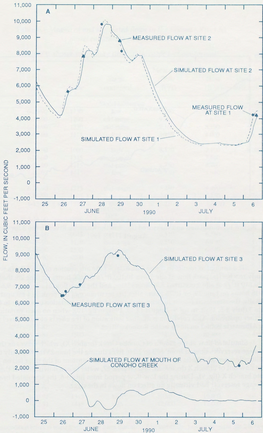
Figure 9.--Simulated and measured flows for the period June 25 through July 6, 1990, at (A) Roanoke River sites 1 and 2, and (B) Roanoke River site 3 and mouth of Conoho Creek.
