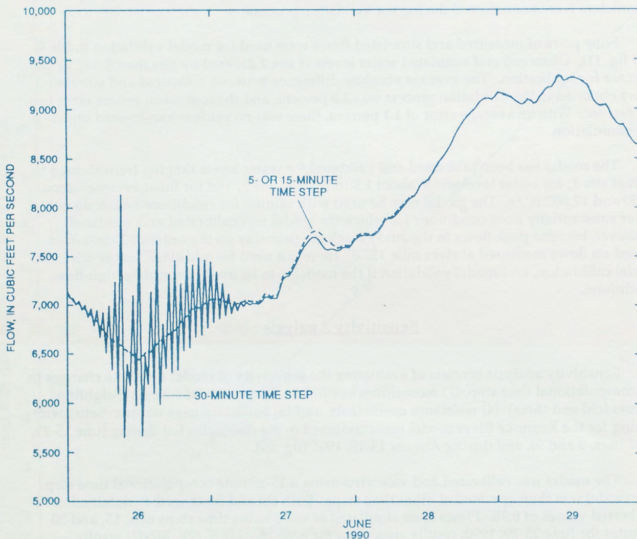
Figure 12.--Simulated flow in the Roanoke River at site 3 for the period June 26-29, 1990, using a 5-, 15-, and 30-minute computational time step.
