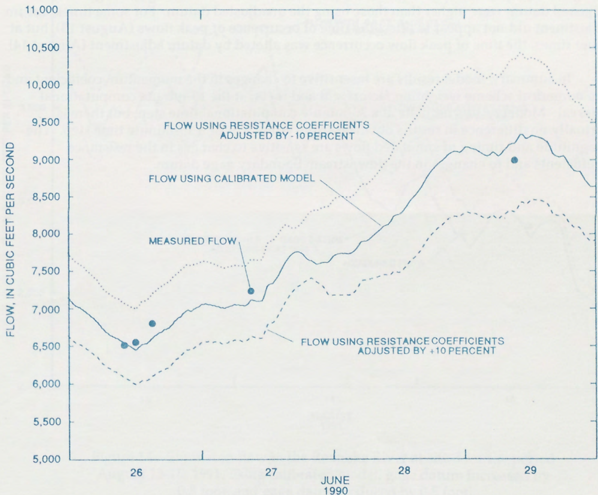
Figure 13.--Simulated flow in the Roanoke River at site 3 for the period June 26-29, 1990, using calibrated model, resistance coefficients increased by 10 percent, and resistance coefficients reduced by 10 percent.
