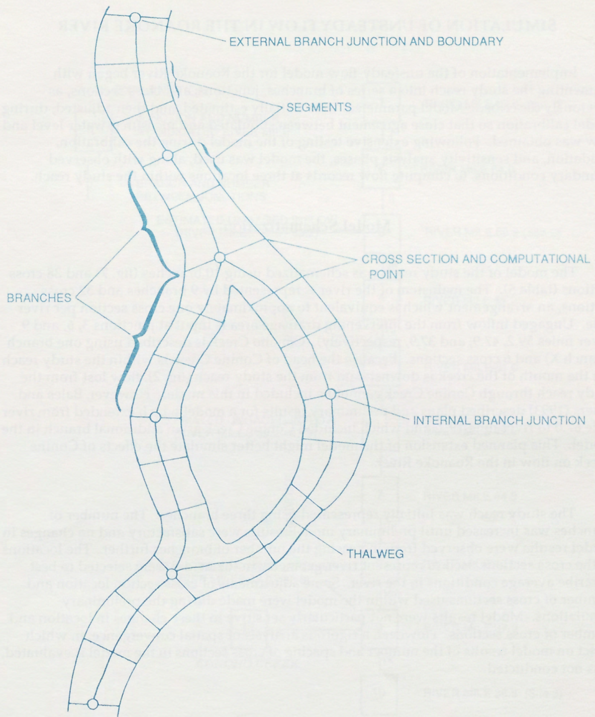
Figure 6.--Idealized branch-network model diagram.
