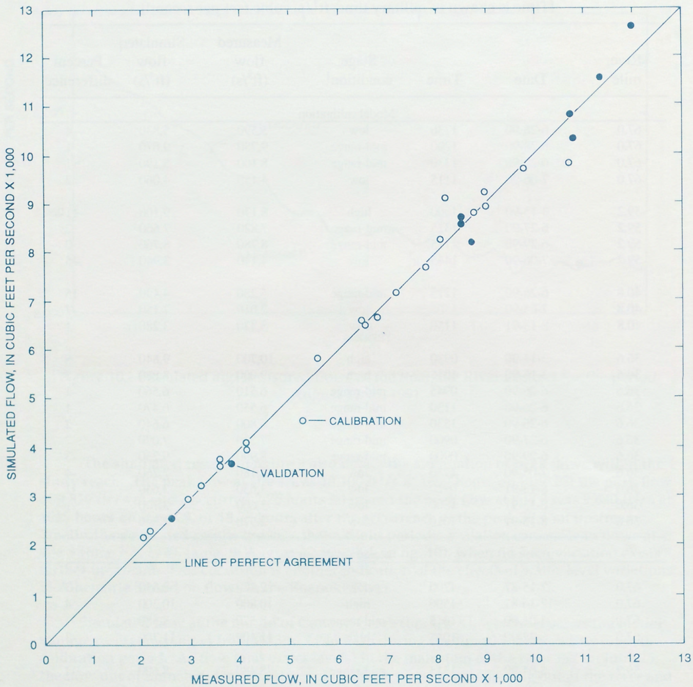
Figure 11.--Relation of simulated and measured flow in the Roanoke River study reach.
