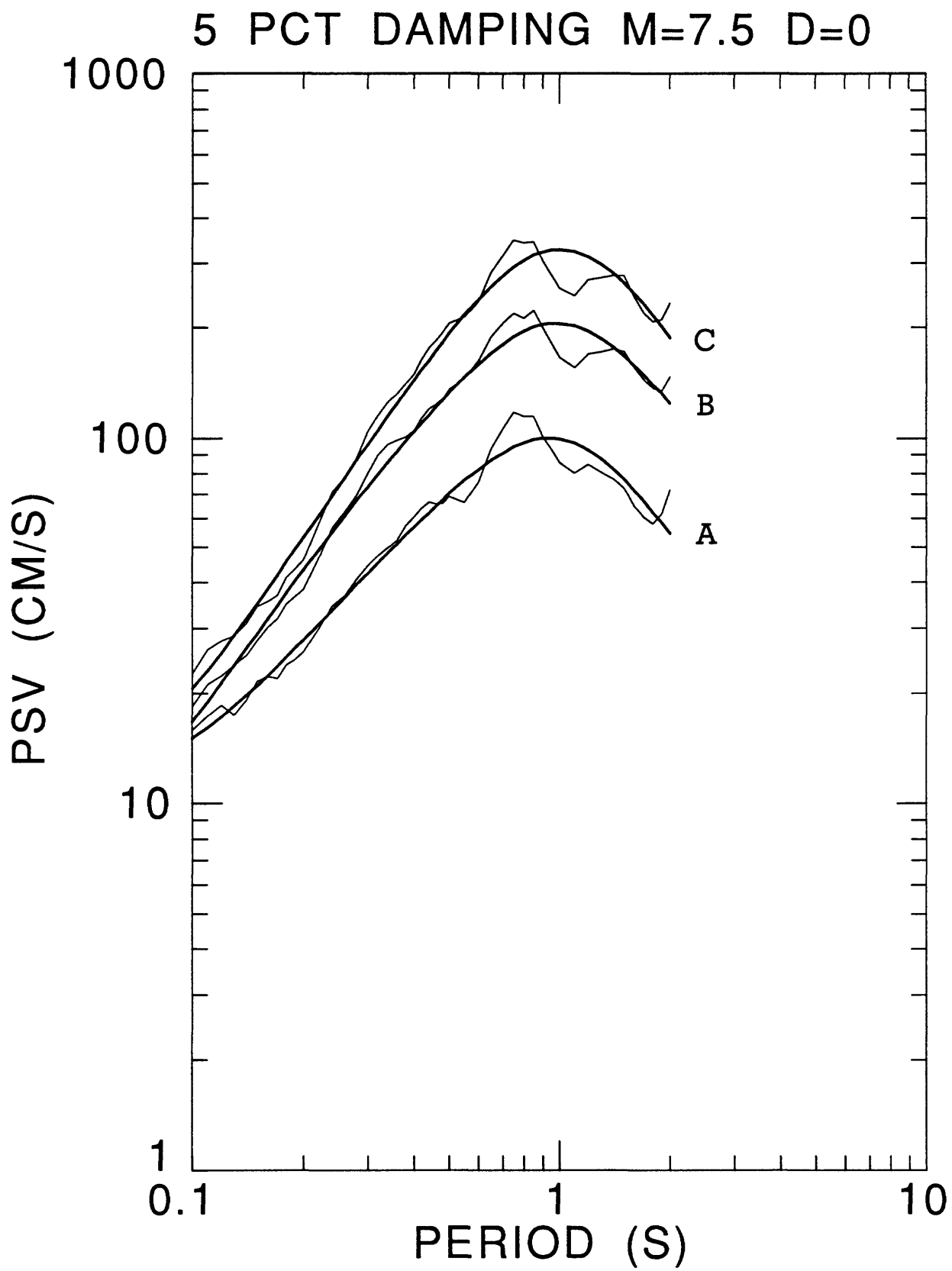
Figure 4. 5 percent damped, random component response spectra for magnitude 7.5 at 0 km distance, predicted from the unsmoothed and smoothed regression coefficients. The three sets of curves are for site classes A, B, and C.
