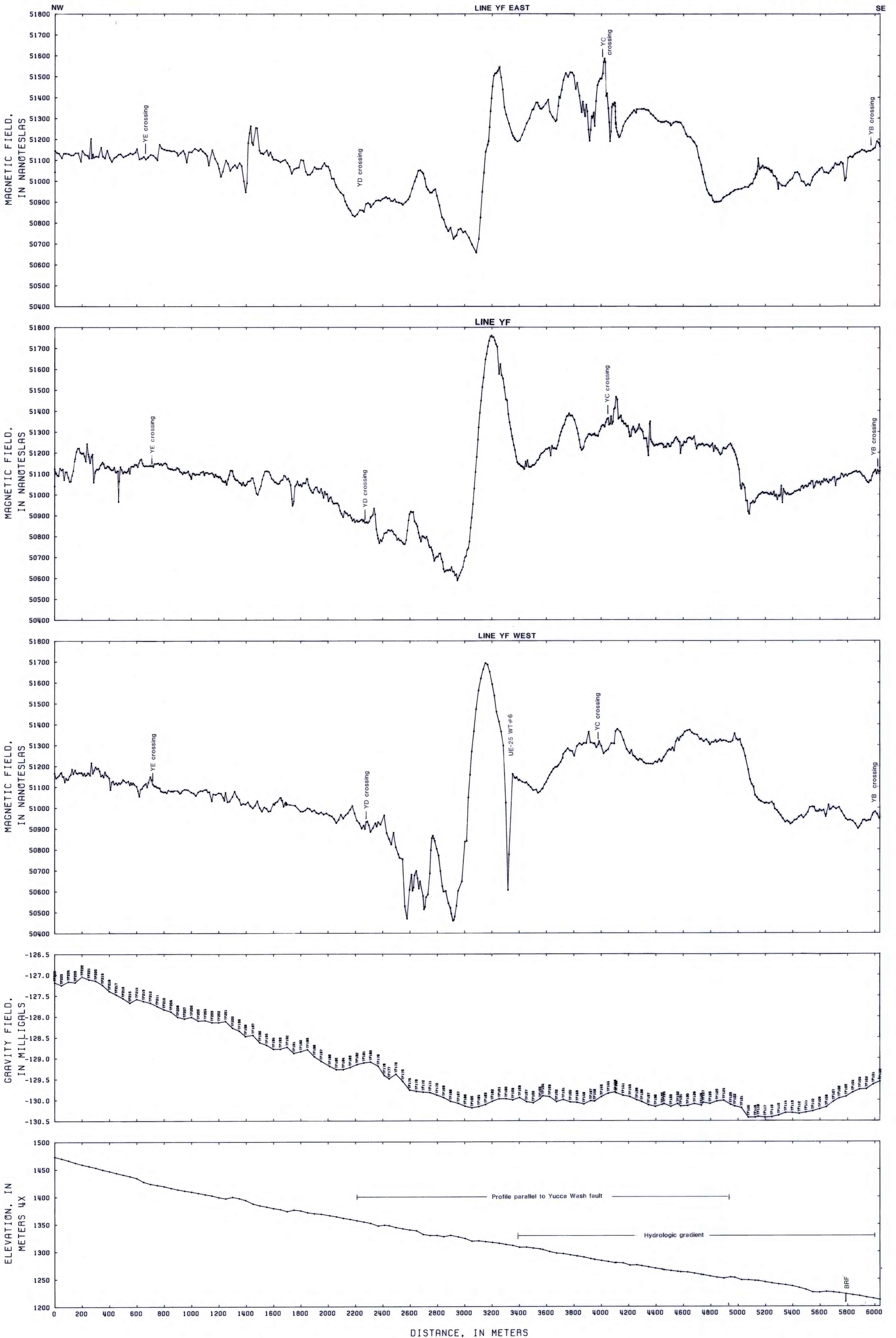
Figure 2f—Gravity, magnetic, and topography profile of line YF and parallel ground magnetic lines approximately 100 m southwest and northeast of line YF. Bouguer gravity anomalies reduced for a density of 2.00 g/cm 3 . Faults shown are from Scott and Bonk (1984). BRF, Bow Ridge fault.
