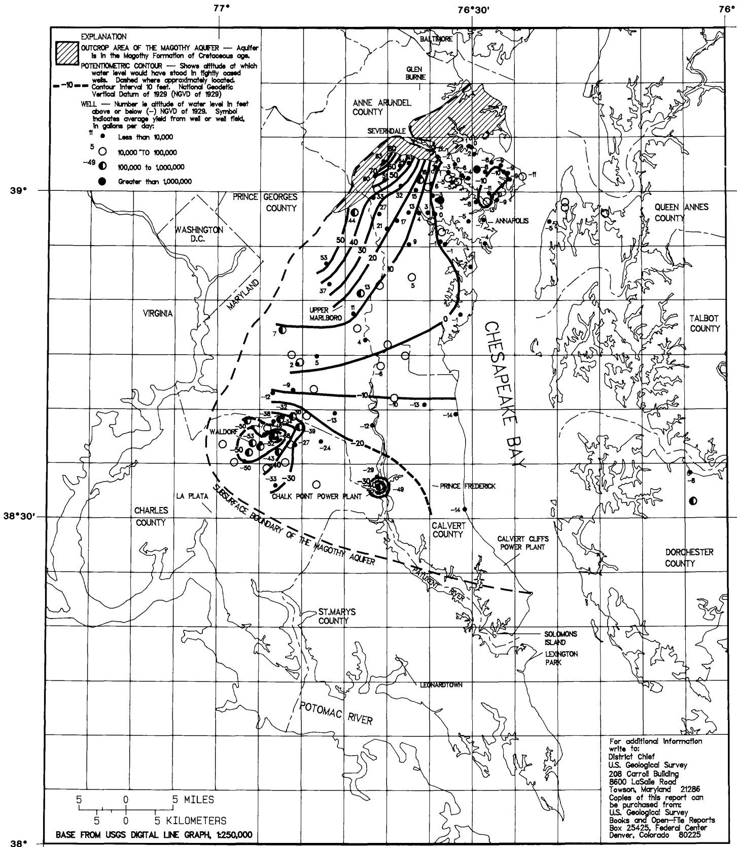
POTENTIOMETRIC SURFACE OF THE MAGOTHY AQUIFER IN SOUTHERN MARYLAND, SEPTEMBER 1991
