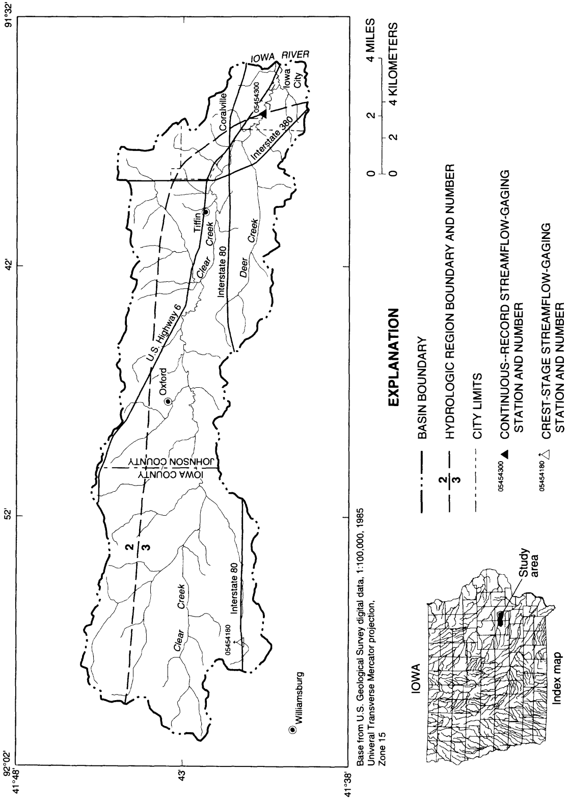
Figure 1. Location of active U.S. Geological Survey streamflow-gaging stations in the Clear Creek Basin.
