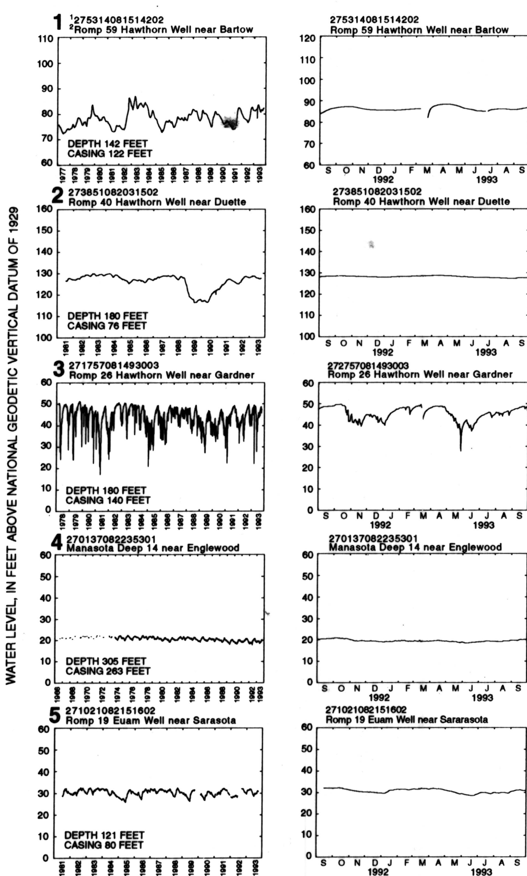
Figure 3.-- Water levels in selected wells tapping the intermediate aquifer system.
