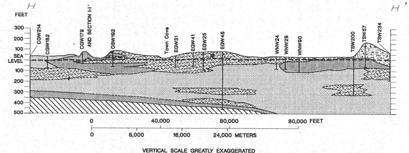
H. Hydrogeologic section H-H'
