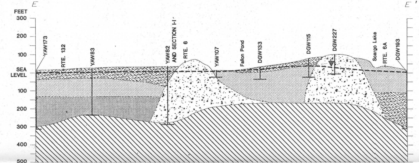
E. Hydrogeologic section E-E'
