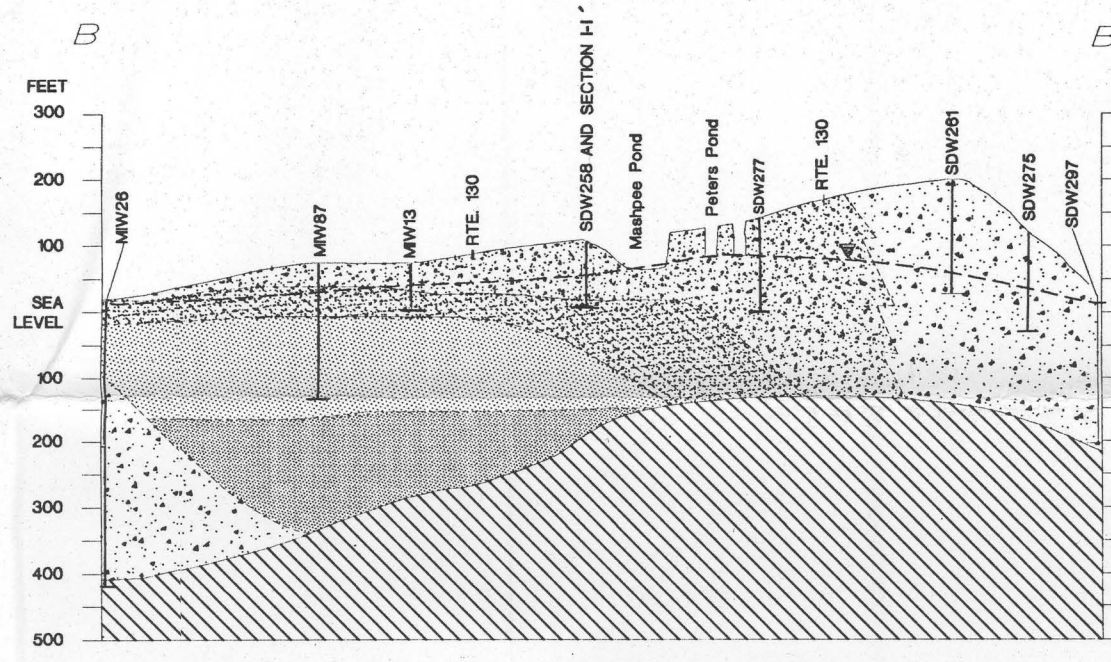
B. Hydrogeologic section B-B'
