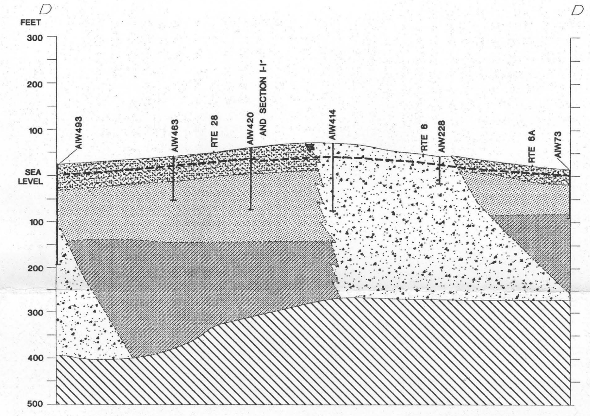
D. Hydrogeologic section D-D'
