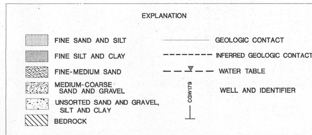
B. Hydrogeologic section B-B'
