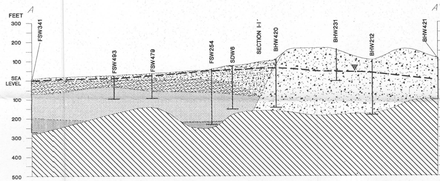
A. Hydrogeologic section A-A'
