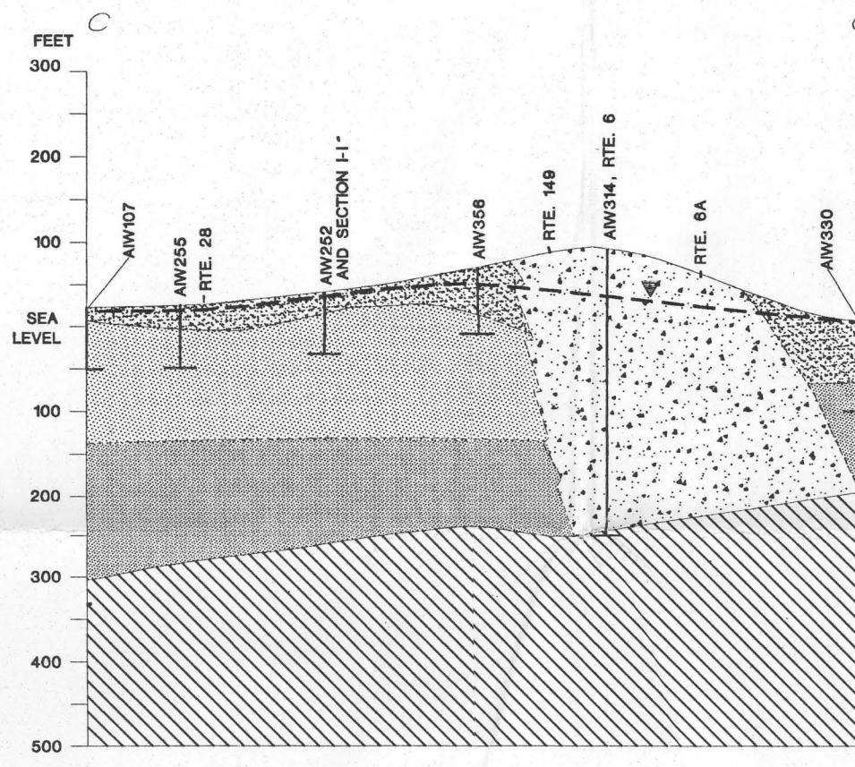
C. Hydrogeologic section C-C'
