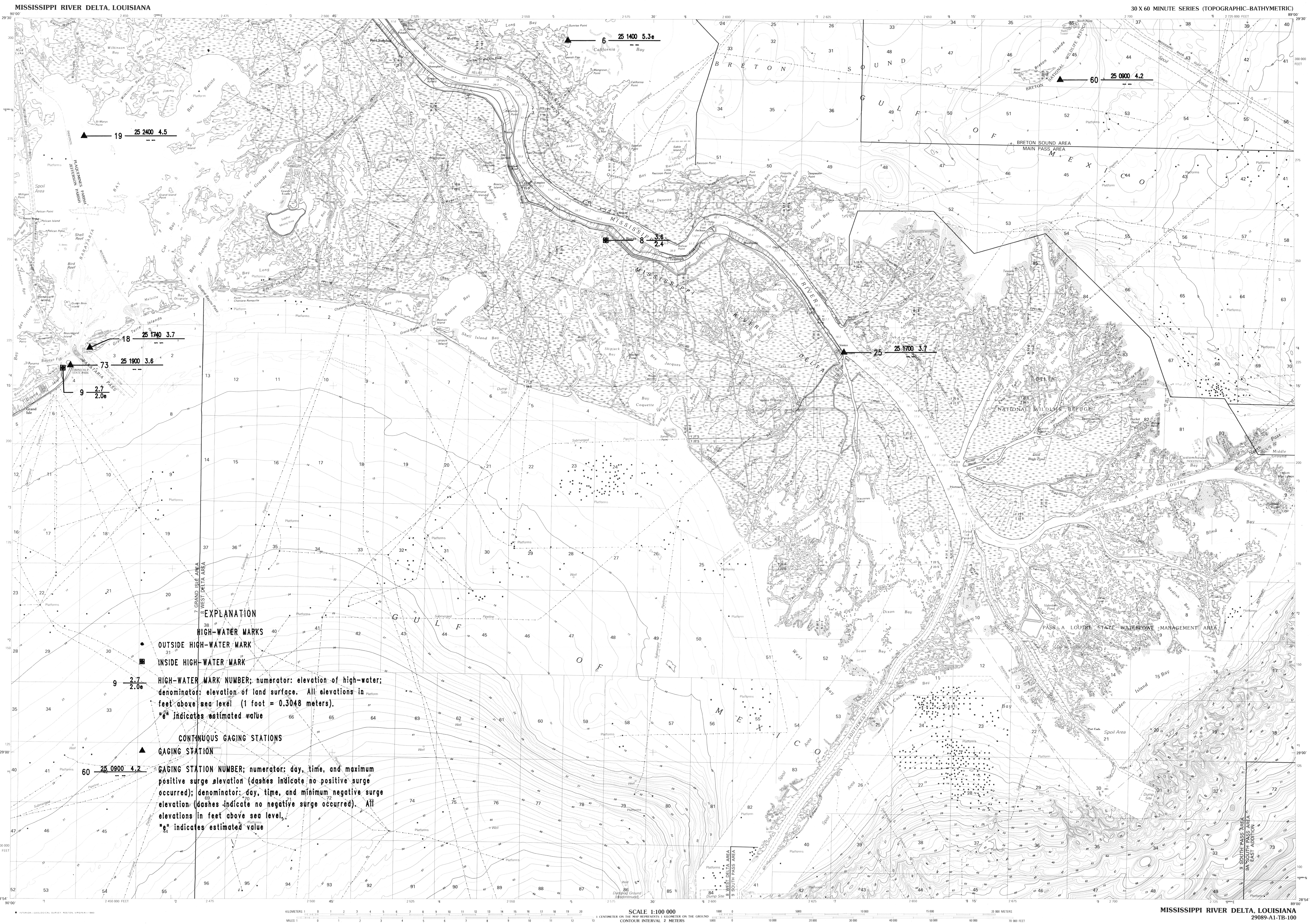
MAP SHOWING HIGH-WATER MARKS, CONTINUOUS GAGING STATIONS, AND WATER-SURFACE ELEVATIONS OF STORM-TIDE INUNDATION CAUSED BY HURRICANE ANDREW, AUGUST 25-27, 1992: MISSISSIPPI RIVER DELTA, LOUISIANA QUADRANGLE
