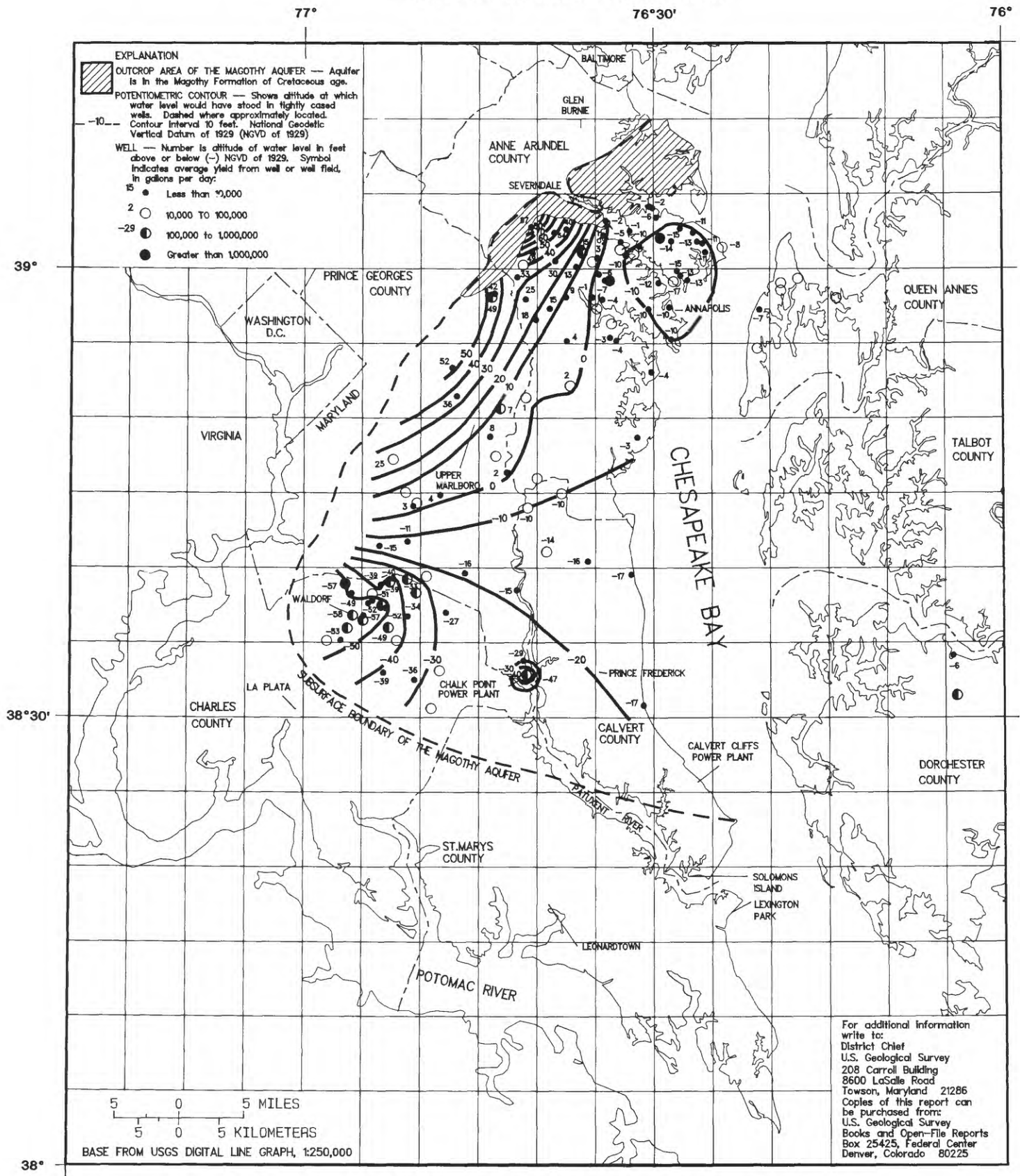
POTENTIOMETRIC SURFACE OF THE MAGOTHY AQUIFER IN SOUTHERN MARYLAND, SEPTEMBER 1993
