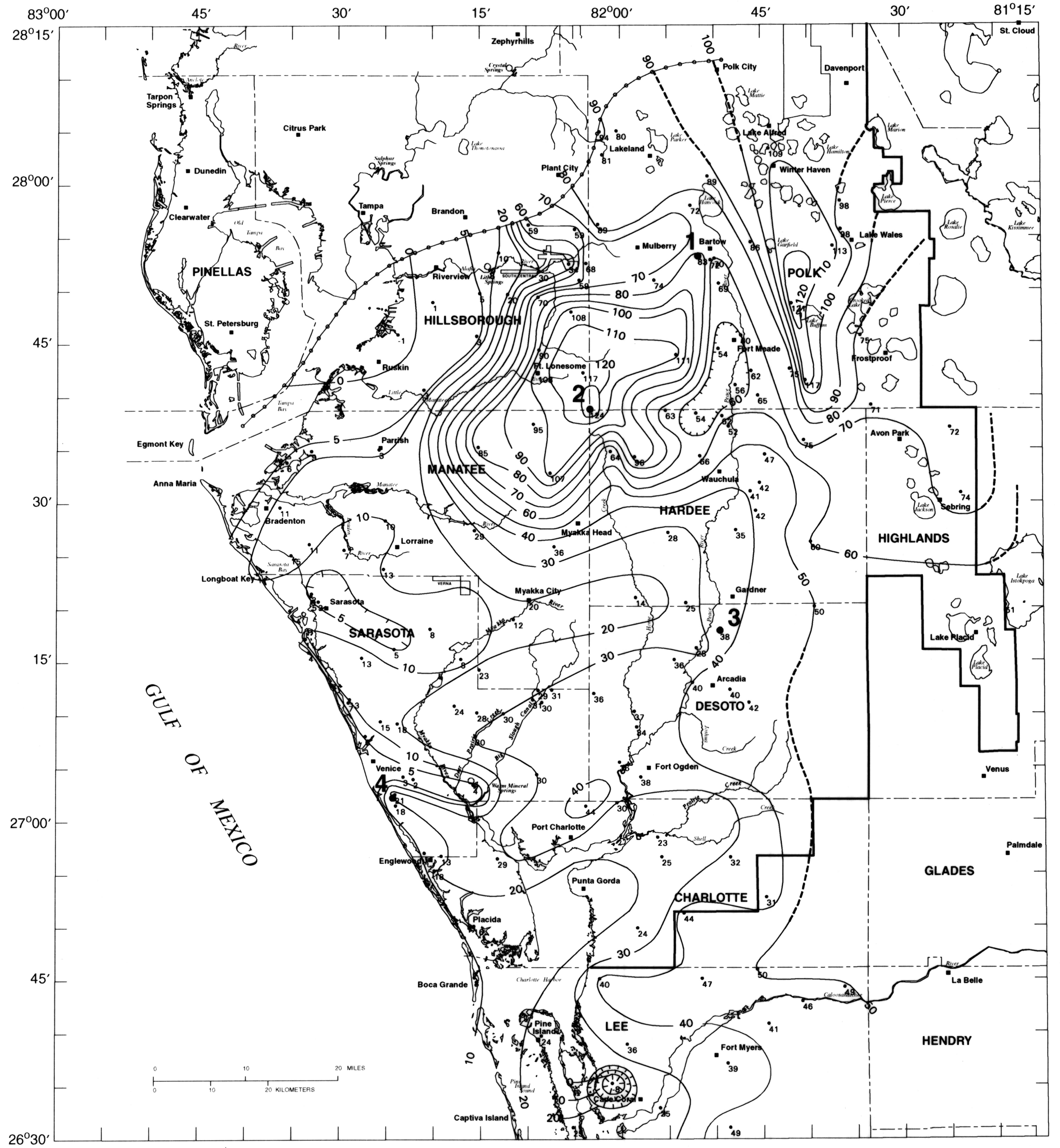
Figure 1. -- Composite potentiometric surface of the intermediate aquifer system.
