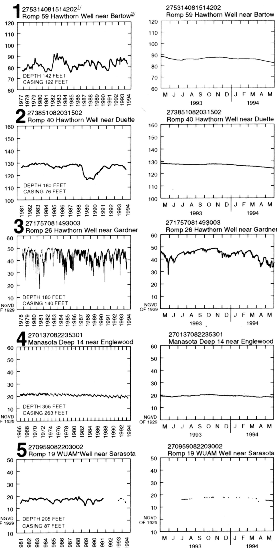
Figure 3. -- Maximum daily water levels in selected wells open to the intermediate aquifer system.
