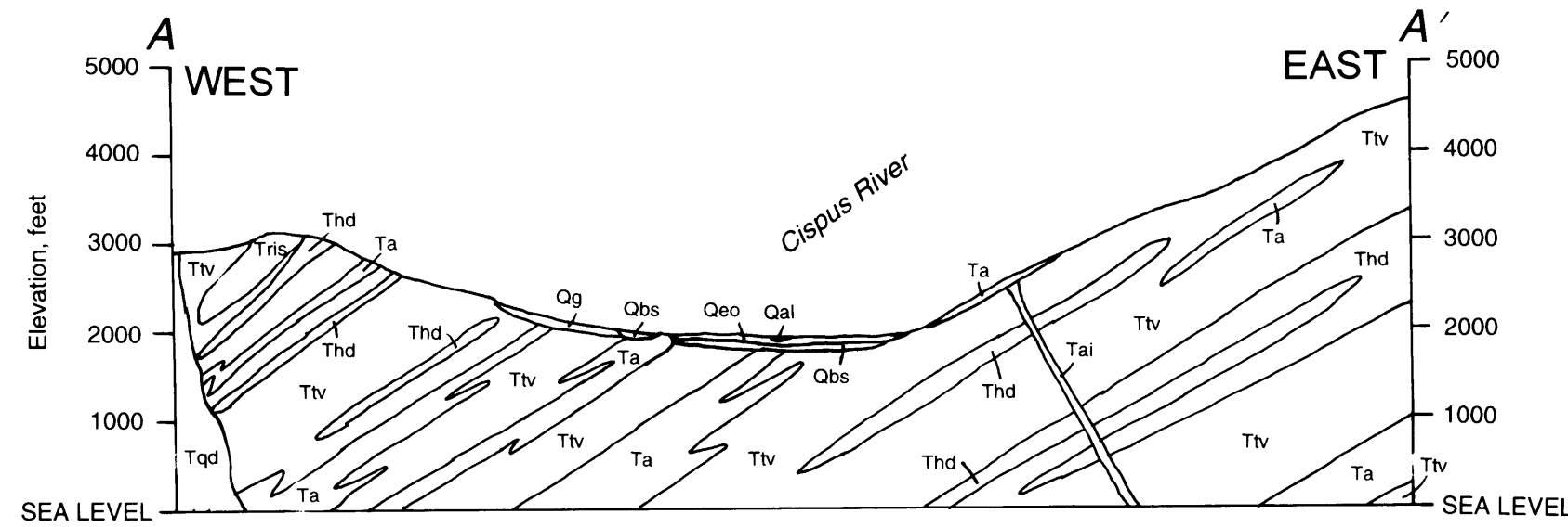
This section connects sections B-B' on McCoy Peak quadrangle and D-D' on Blue Lake quadrangle
