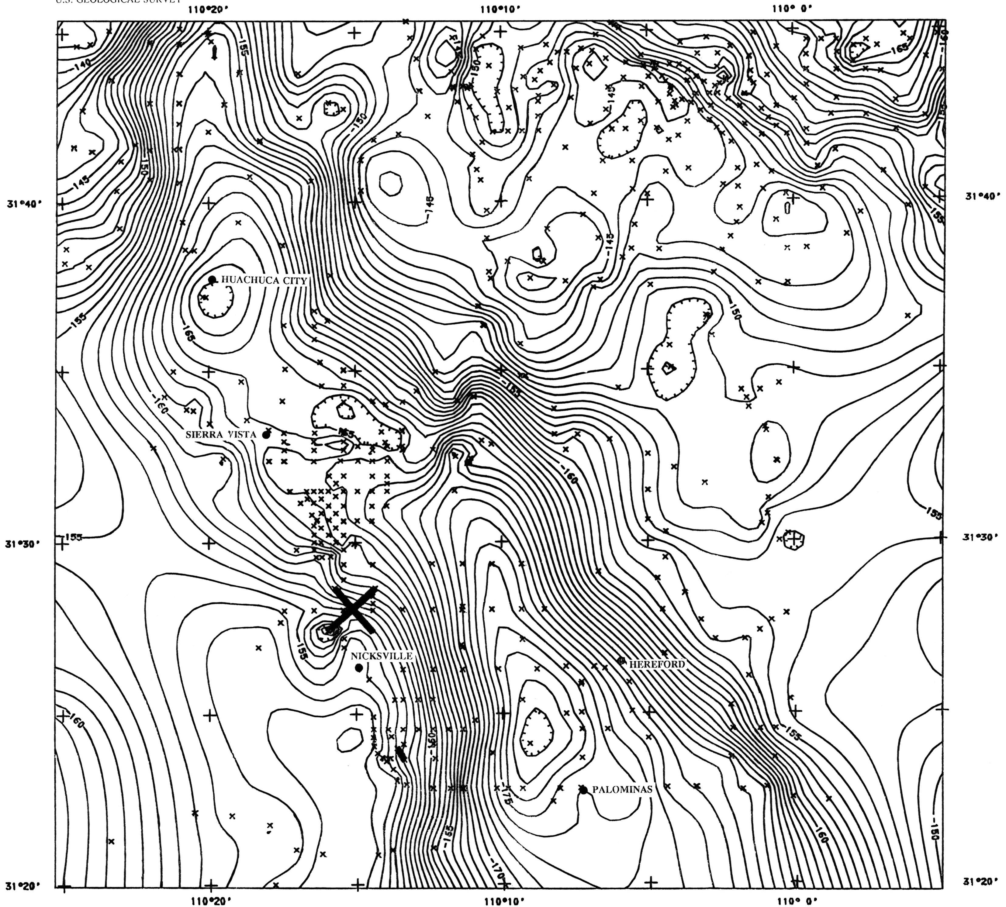
Figure 2. - Complete Bouguer gravity anomaly map of part of the upper San Pedro Valley area. Contour interval for gravity anomaly values is 1 mgal and hachured contours indicate a relative gravity minimum. Gravity stations are marked by an X. Scale is 1:125,000.
