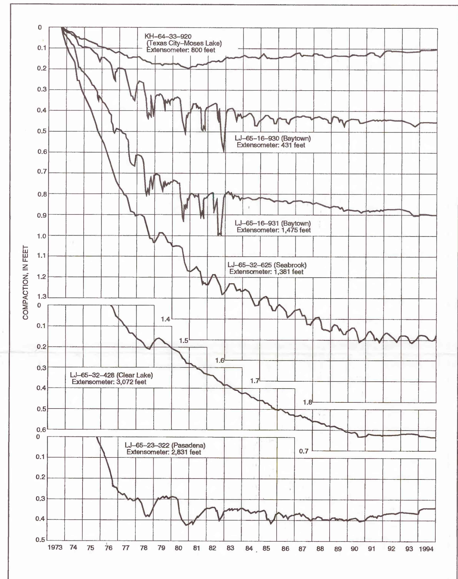
Figure 8. Graphs showing measured compaction of subsurface material, 1973-94, in extensometers shown in figure 7.
