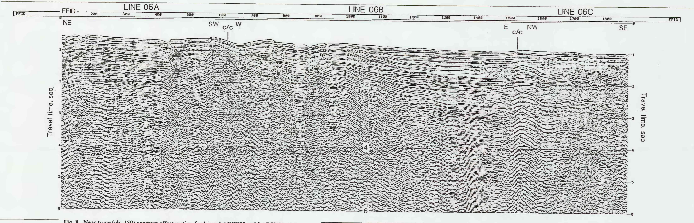
Fig. 8. Near-trace (ch. 150) constant offset section for Lines LARSE03 and LARSE06. As described in text processing included band pass filtering, automatic gain control (AGC), and water column mute.
