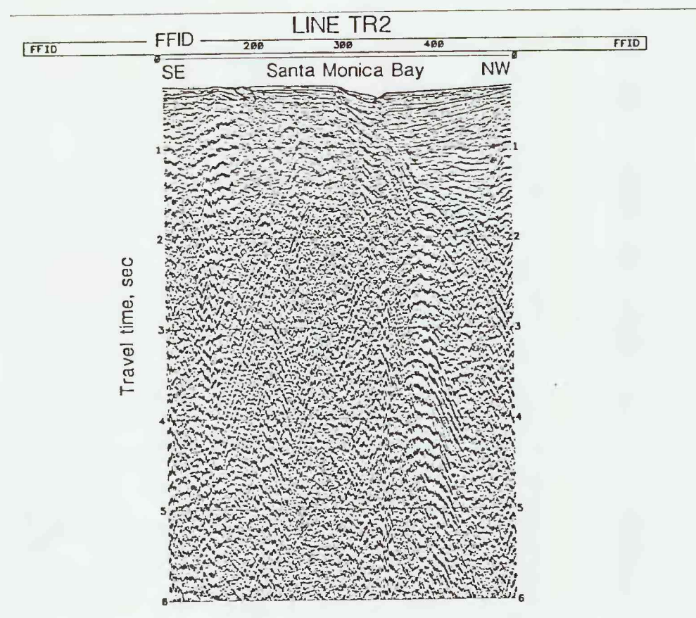
Fig. 9. Near-trace (ch. 150) constant offset section for Lines TR1a and b, TR2, and TR3. As described in text processing included band pass filtering, automatic gain control (AGC), and water column mute.
