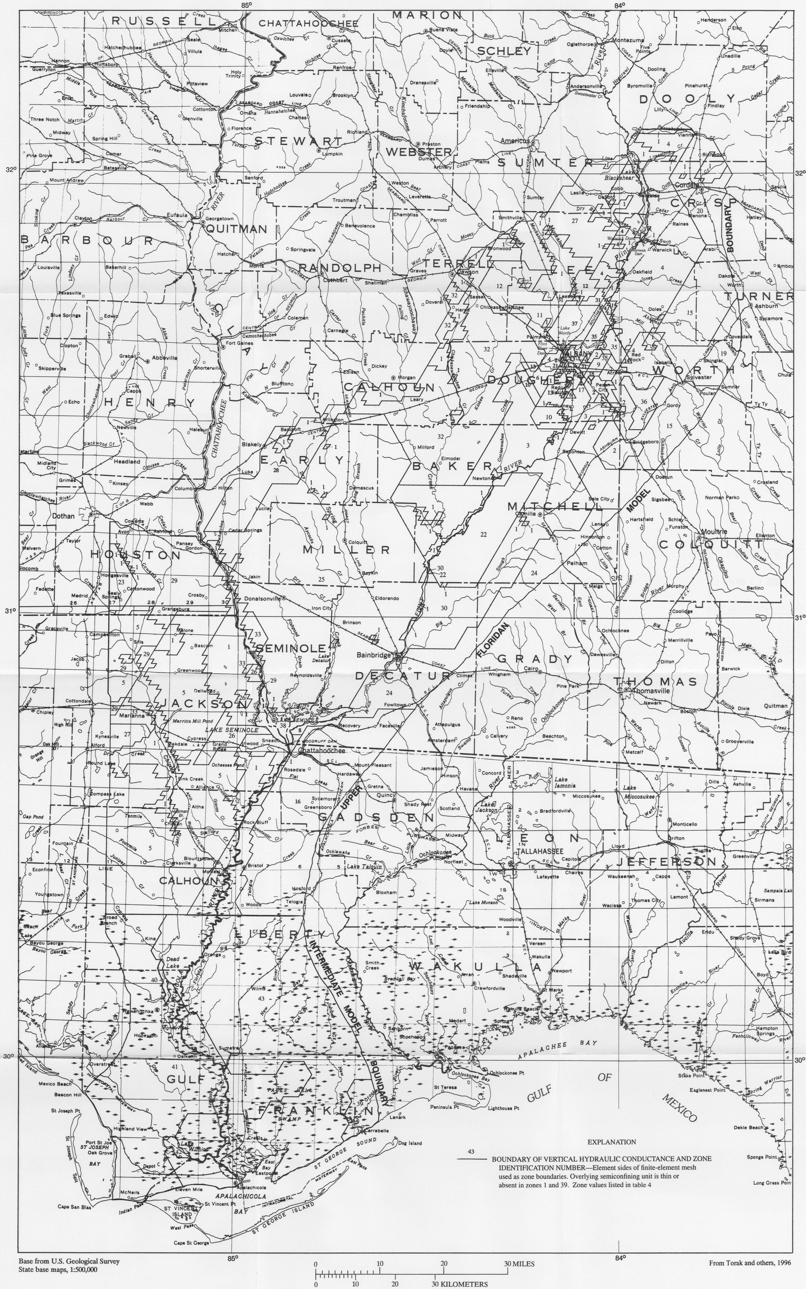
MAP SHOWING ZONES OF VERTICAL HYDRAULIC CONDUCTANCE OF OVERLYING SEMICONFINING UNITS IN THE UPPER FLORIDAN AND INTERMEDIATE MODELS IN THE LOWER APALACHICOLA-CHATTAHOOCHEE-FLINT RIVER BASIN, SOUTHEASTERN ALABAMA, NORTHWESTERN FLORIDA, AND SOUTHWESTERN GEORGIA
