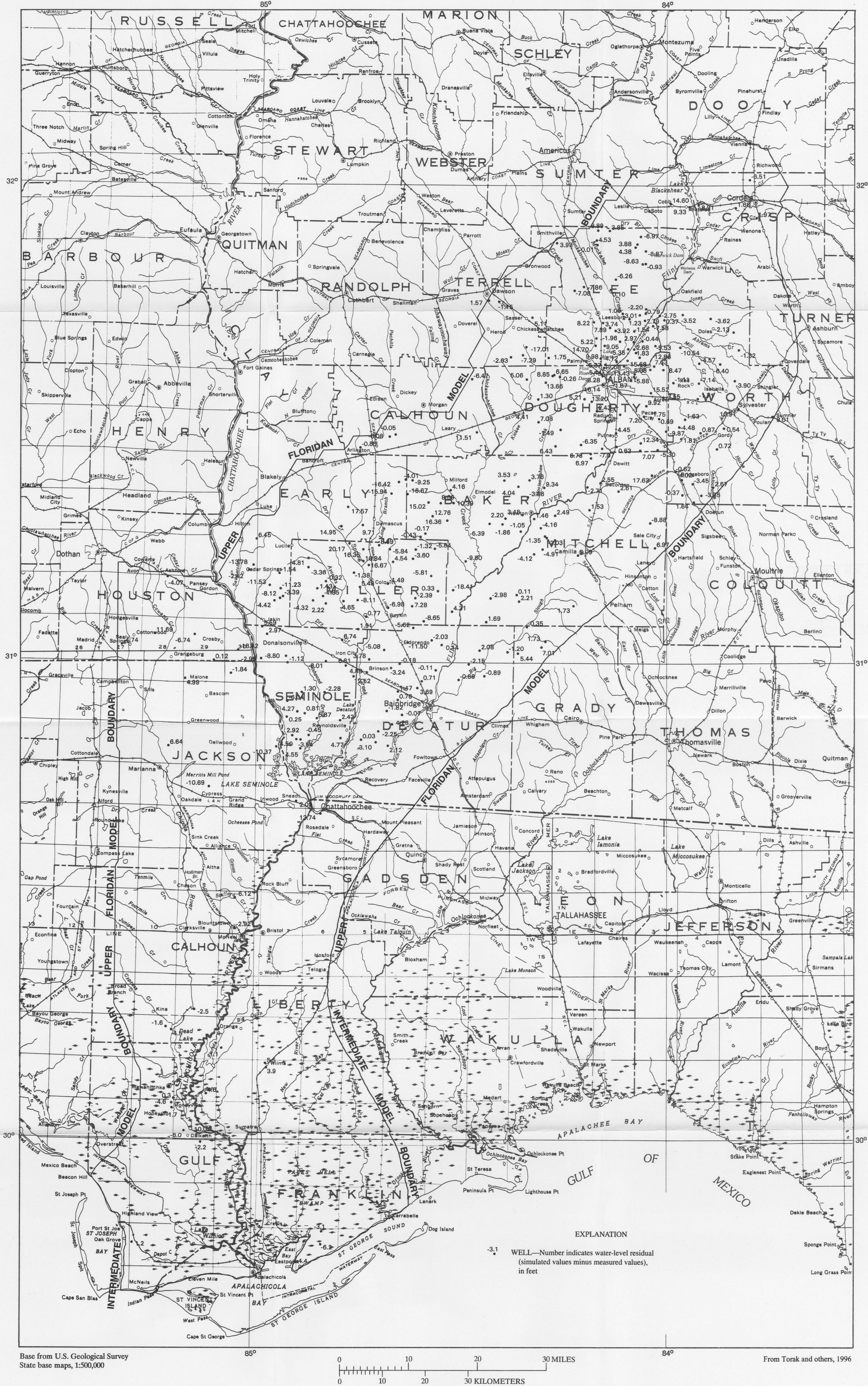
MAP SHOWING LOCATIONS OF WATER-LEVEL MEASUREMENTS AND WATER-LEVEL RESIDUALS FOR THE CALIBRATED UPPER FLORIDAN AND INTERMEDIATE MODELS IN THE LOWER APALACHICOLA-CHATAHOOCHEE-FLINT RIVER BASIN, SOUTHEASTERN ALABAMA, NORTHWESTERN FLORIDA, AND SOUTHWESTERN GEORGIA, OCTOBER 1986
