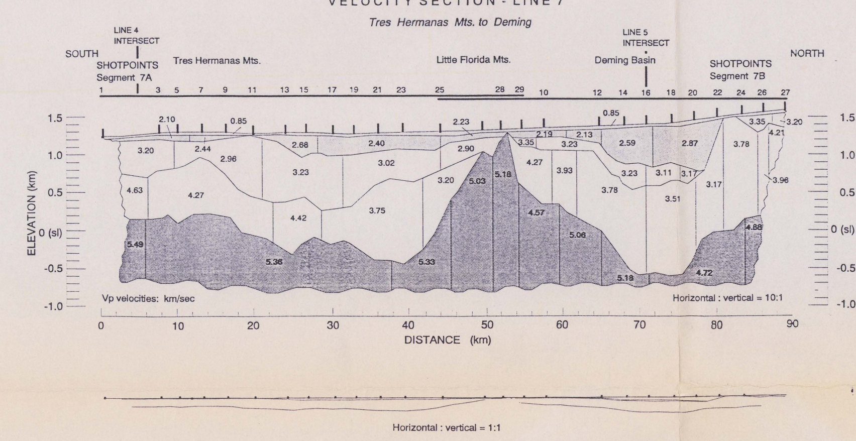
STRUCTURE OF THE BASINS AND RANGES, SOUTHWEST NEW MEXICO, AN INTERPRETATION OF SEISMIC VELOCITY SECTIONS
