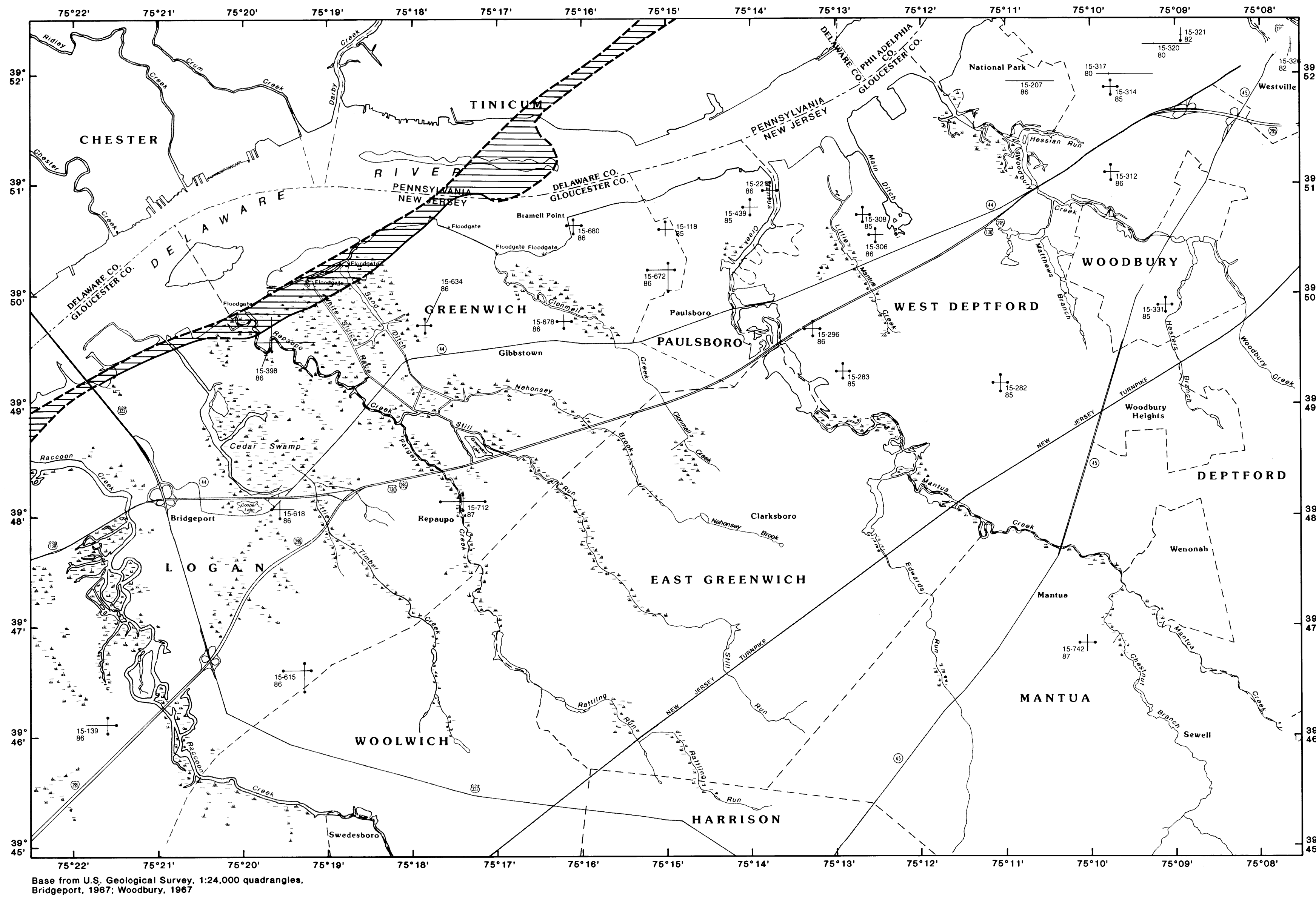
A. DISTRIBUTION OF DISSOLVED ARSENIC, CADMIUM, CHROMIUM, AND LEAD IN WATER IN THE LOWER AQUIFER OF THE POTOMAC-RARITAN-MAGOTHY AQUIFER SYSTEM IN THE REGION OF GREENWICH TOWNSHIP, GLOUCESTER COUNTY, NEW JERSEY, 1980-88
