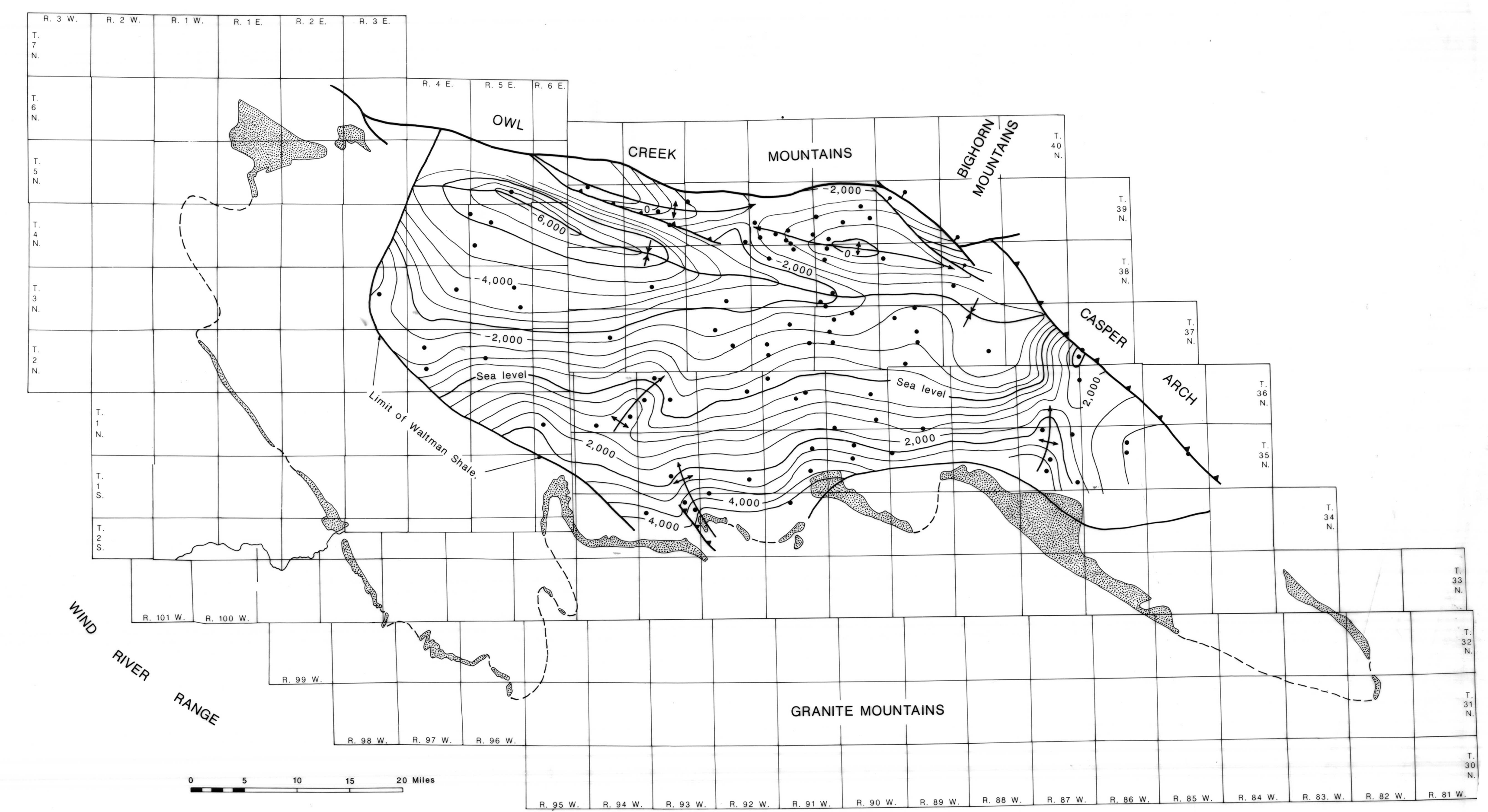
Plate 1d: Base of Waltman Shale Member of the Fort Union Formation.
