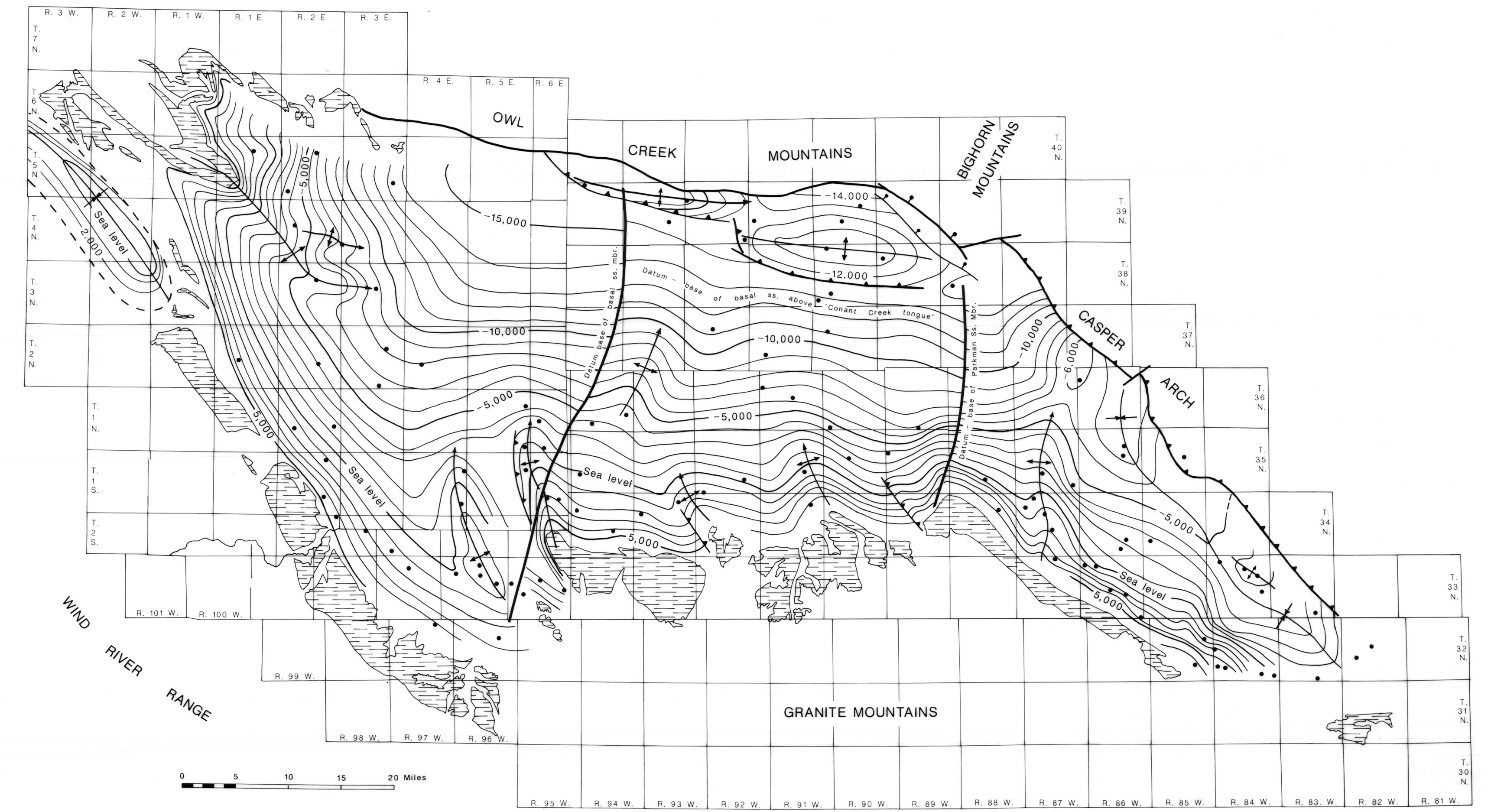
Plate 1b: Top of Cody Shale. Position of Casper arch thrust at top of Cody is modified from Skeen and Ray (1983, Figure 23).
