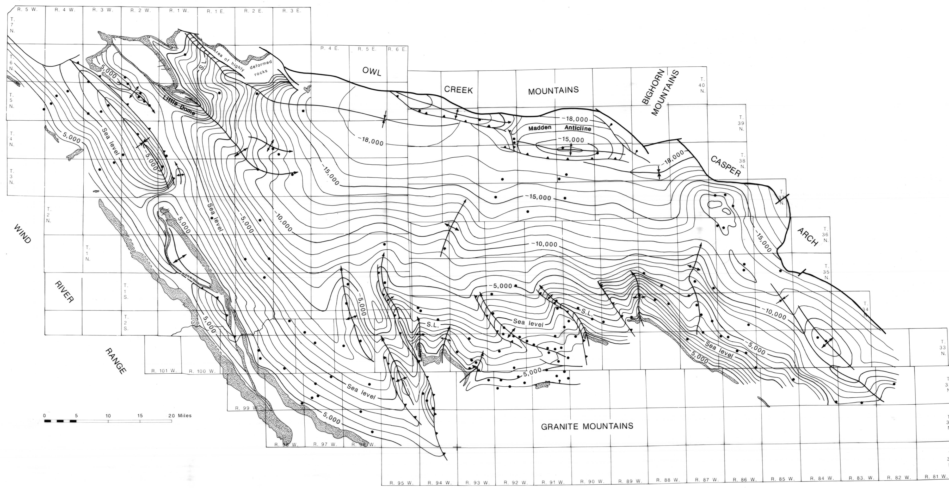
Plate 1a: Top of Frontier Formation. Contours on footwall of Casper arch thrust and position of Casper arch thrust at the Frontier level are modified from Skeen and Ray (1983, Figure 23). The map extends to the north to a series of normal faults that cut the Owl Creek thrust along the south flank of the Owl Creek Mountains (see Keefer, 1970, Plate 1).
