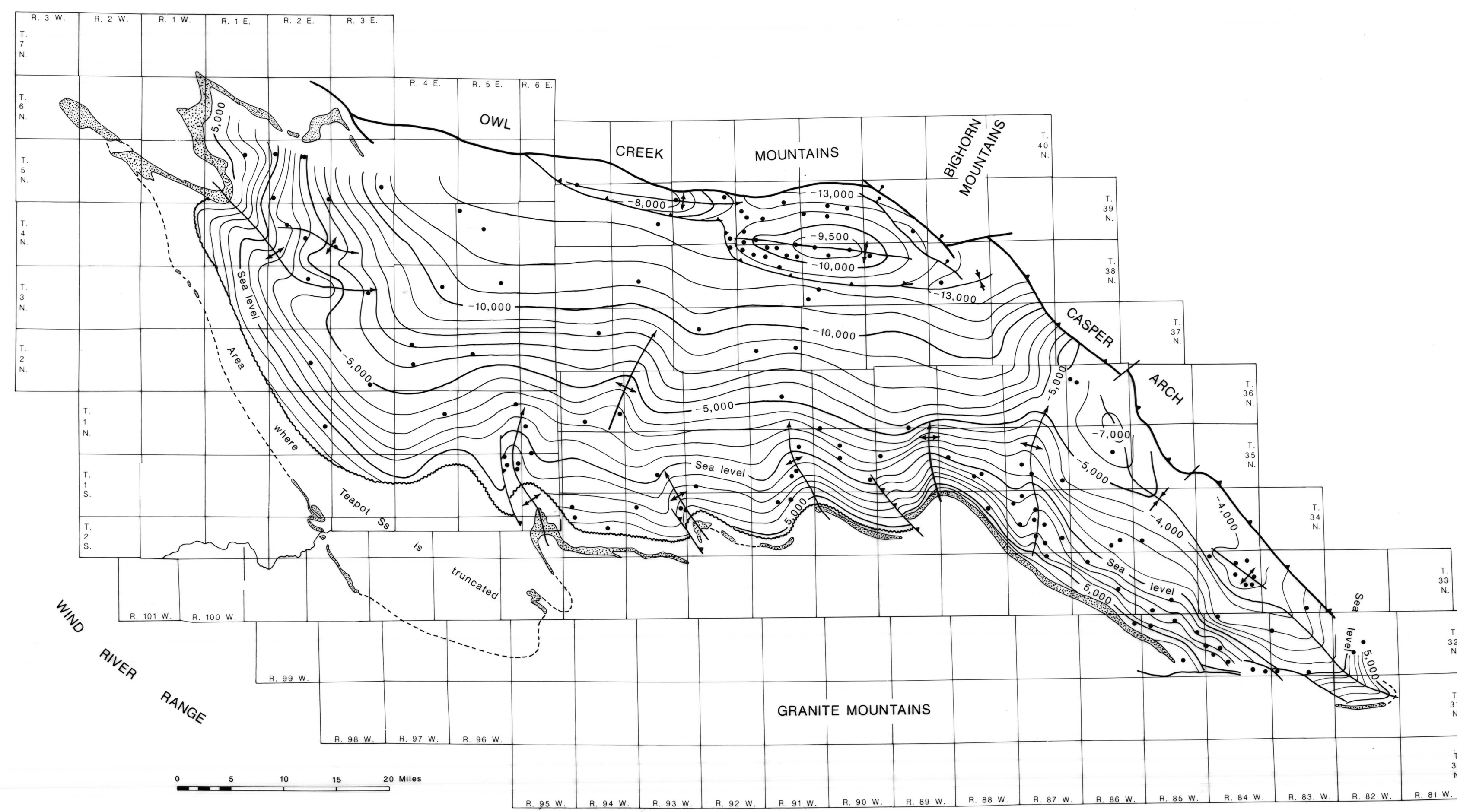
Plate 1c: Top of Teapot Sandstone Member of the Mesaverde Formation. Position of Casper arch thrust Teapot Sandstone is modified from Skeen and Ray (1983, Figure 23).
