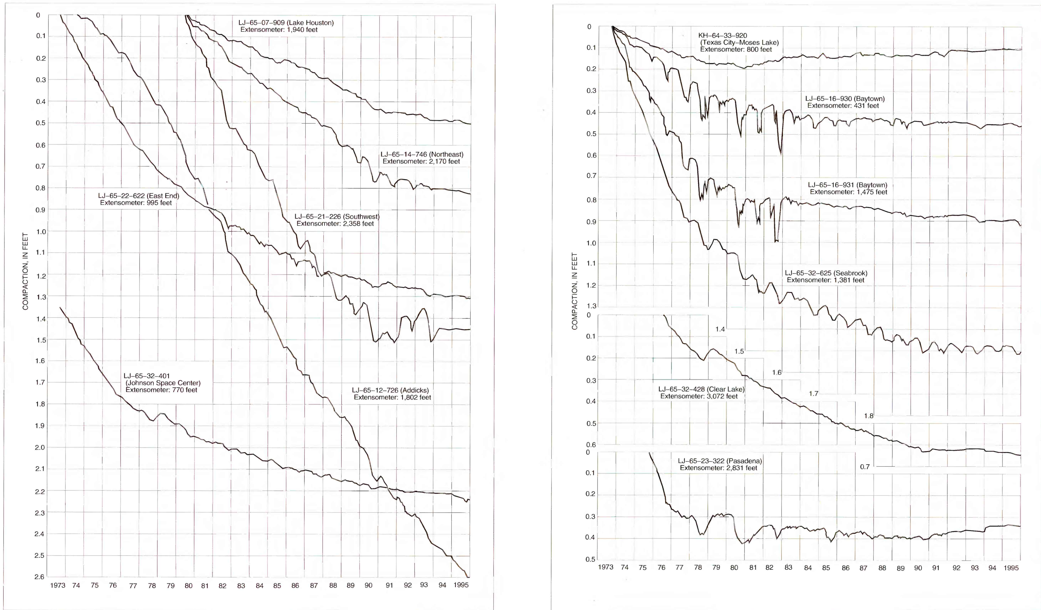
Figure 8. Graphs showing measured compaction of subsurface material, 1973-95, in extensometers shown in figure 7.
