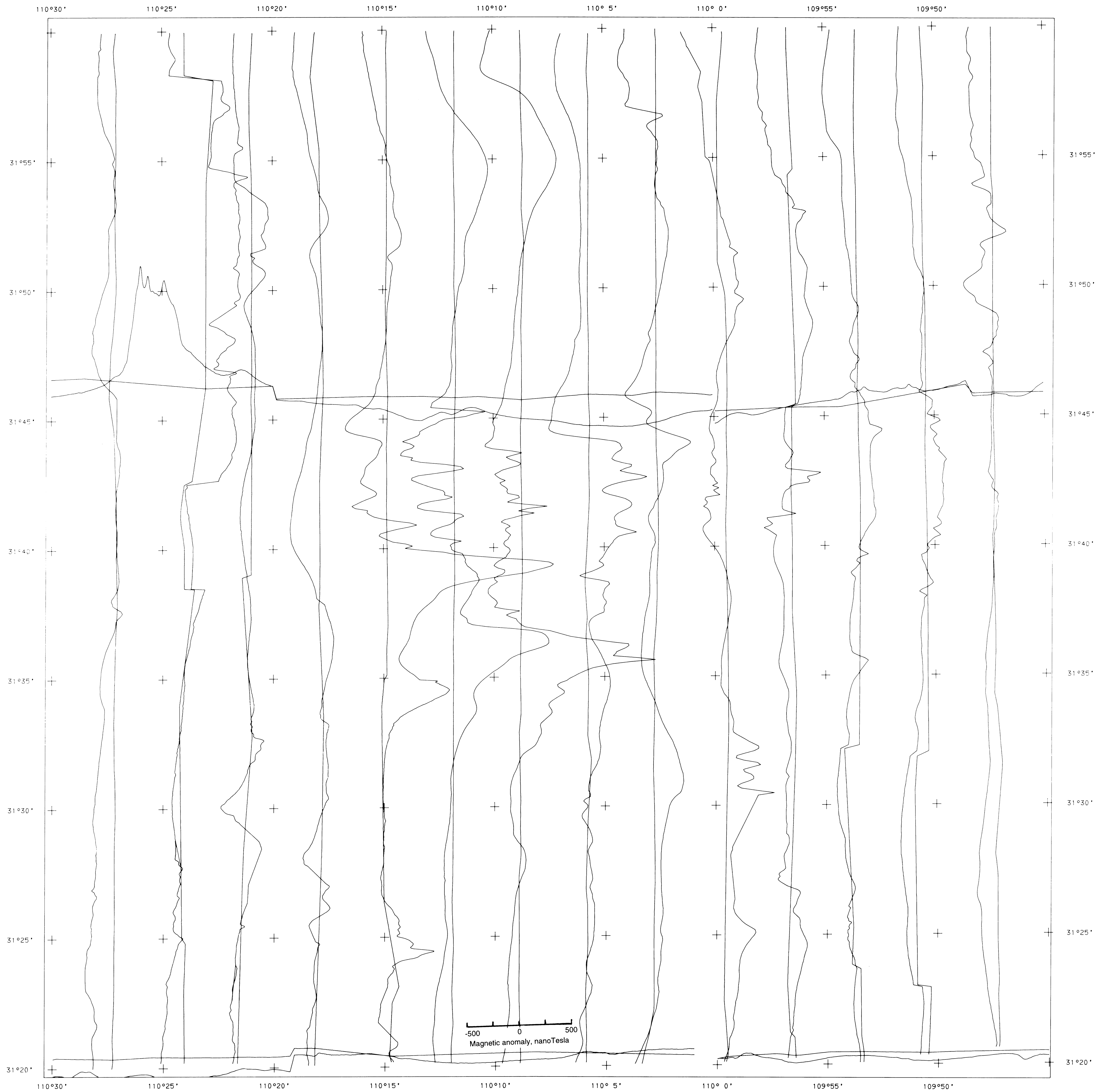
Plate 3. NURE aeromagnetic total field intensity anomaly profiles in the San Pedro Valley area. Nominal ground clearance is 400 ft (122m). Anomaly profile values are plotted relative to flight line path at a scale of 250 nT/minute of latitude.
