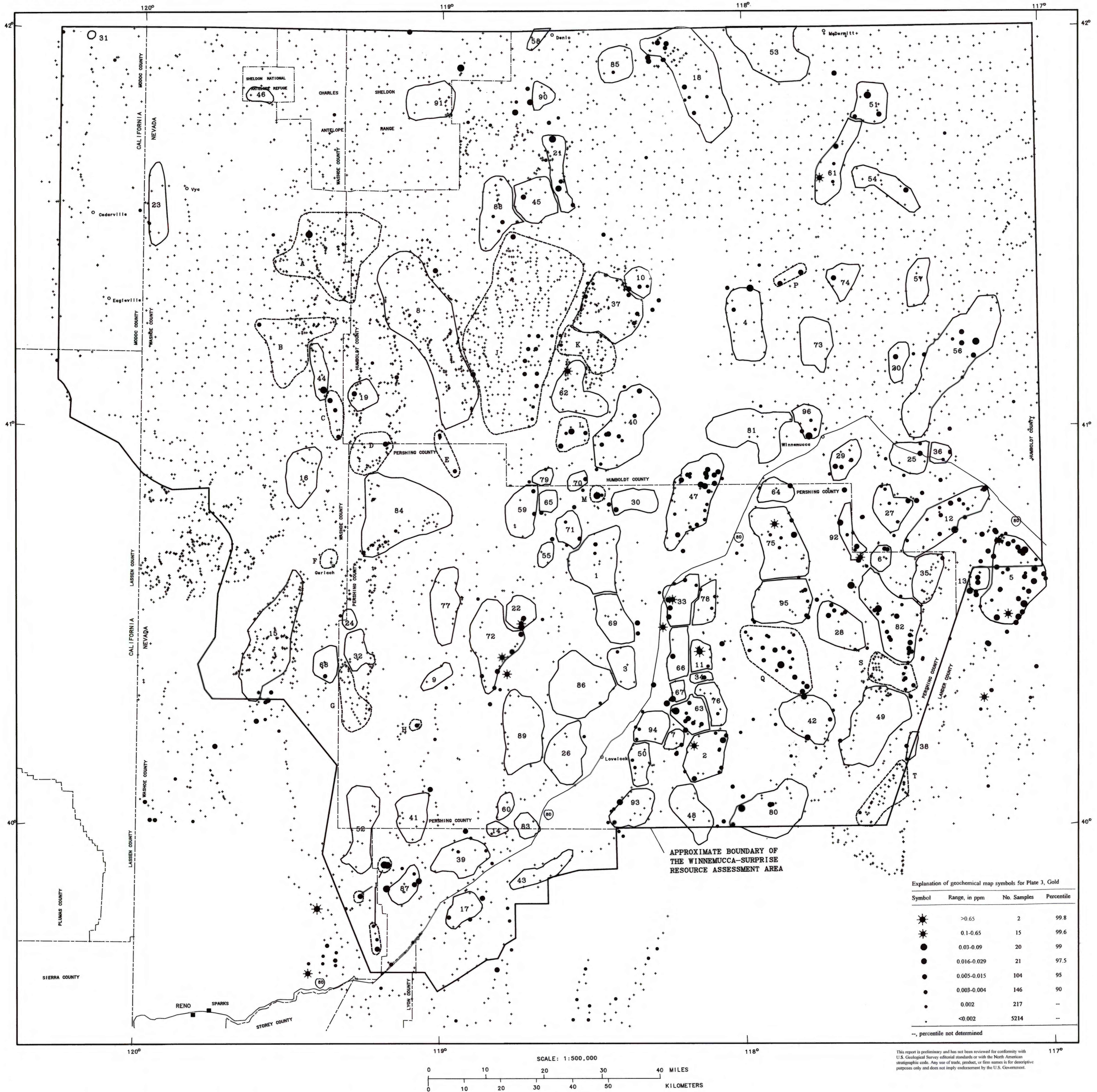
GEOCHEMICAL MAP SHOWING DISTRIBUTION AND ABUNDANCE OF GOLD IN STREAM-SEDIMENT AND SOIL SAMPLES IN THE WINNEMUCCA-SURPRISE RESOURCE ASSESSMENT AREA, NORTHWEST NEVADA AND NORTHEAST CALIFORNIA
