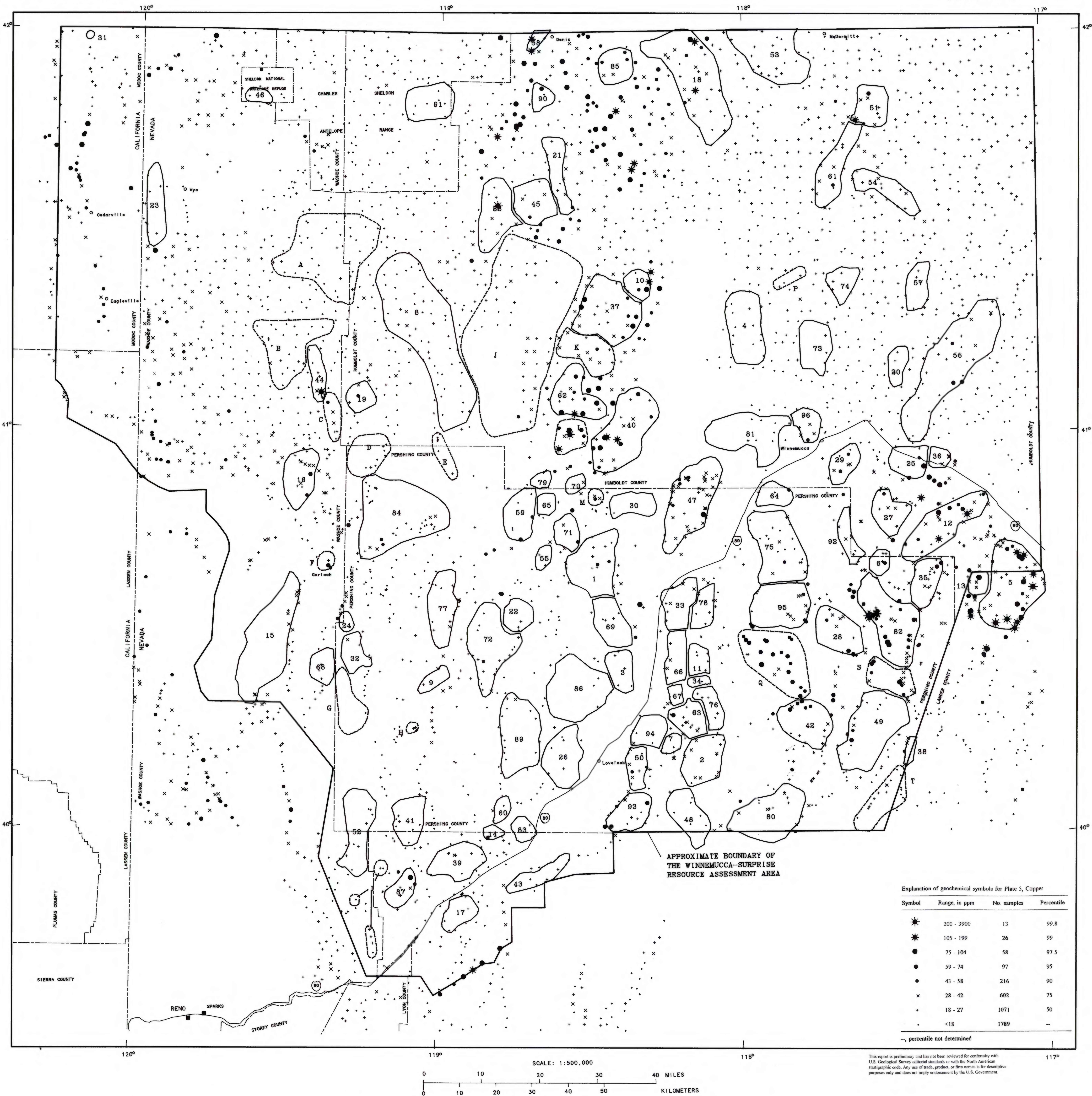
GEOCHEMICAL MAP SHOWING DISTRIBUTION AND ABUNDANCE OF COPPER IN STREAM-SEDIMENT AND SOIL SAMPLES IN THE WINNEMUCCA-SURPRISE RESOURCE ASSESSMENT AREA, NORTHWEST NEVADA AND NORTHEAST CALIFORNIA
