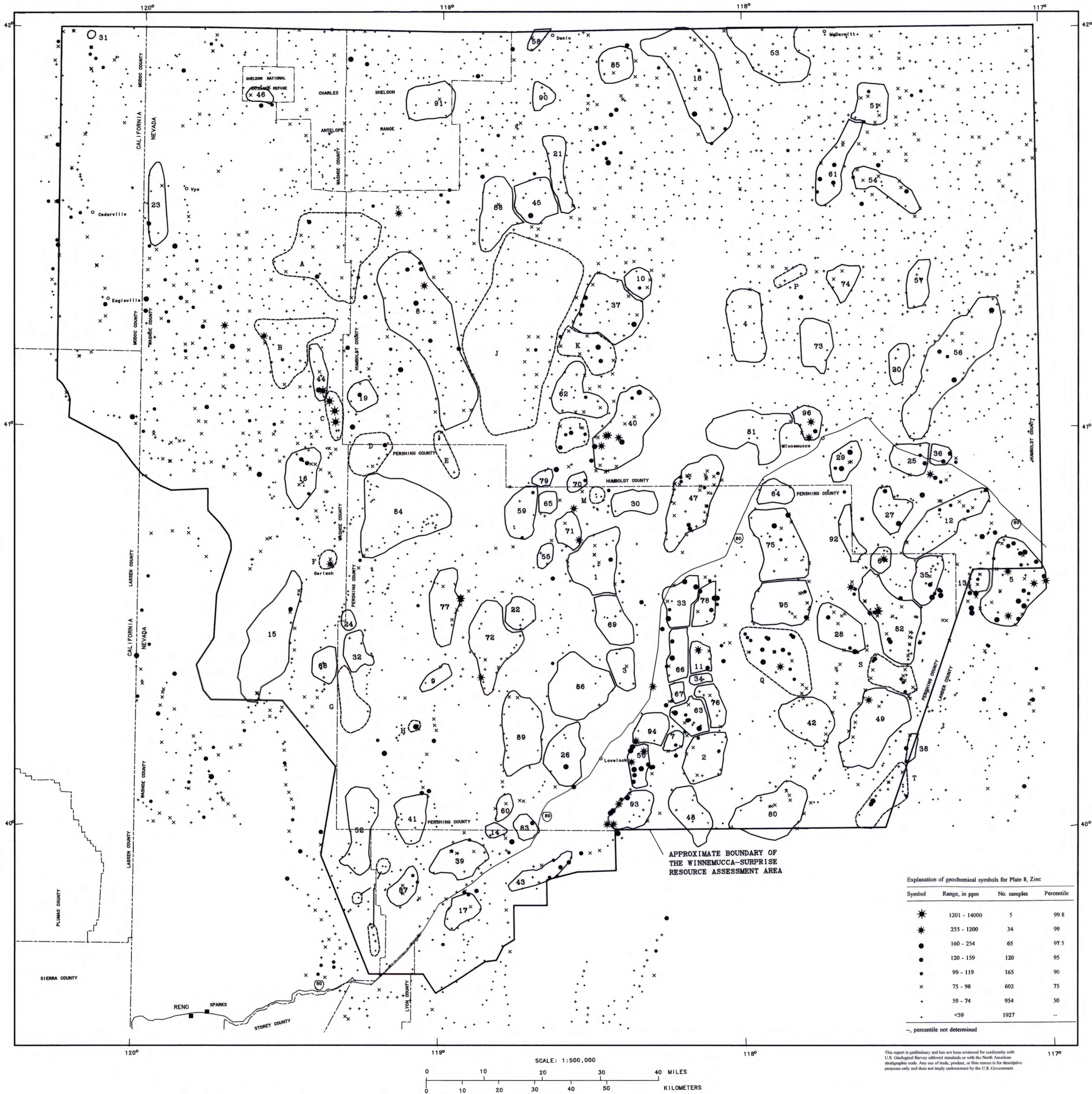
GEOCHEMICAL MAP SHOWING DISTRIBUTION AND ABUNDANCE OF ZINC IN STREAM-SEDIMENT AND SOIL SAMPLES IN THE WINNEMUCCA-SURPRISE RESOURCE ASSESSMENT AREA, NORTHWEST NEVADA AND NORTHEAST CALIFORNIA INTERPRETATION OF RECONNAISSANCE GEOCHEMICAL DATA FROM THE BUREAU OF LAND MANAGEMENT'S WINNEMUCCA DISTRICT AND SURPRISE RESOURCE AREA, NORTHWEST NEVADA AND NORTHEAST CALIFORNIA
