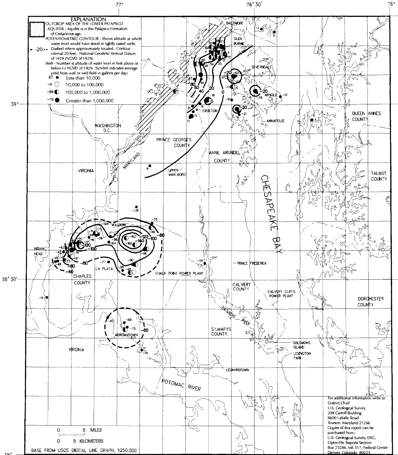
POTENTIOMETRIC SURFACE OF THE LOWER PATAPSCO AQUIFER IN SOUTHERN MARYLAND, SEPTEMBER 1995
