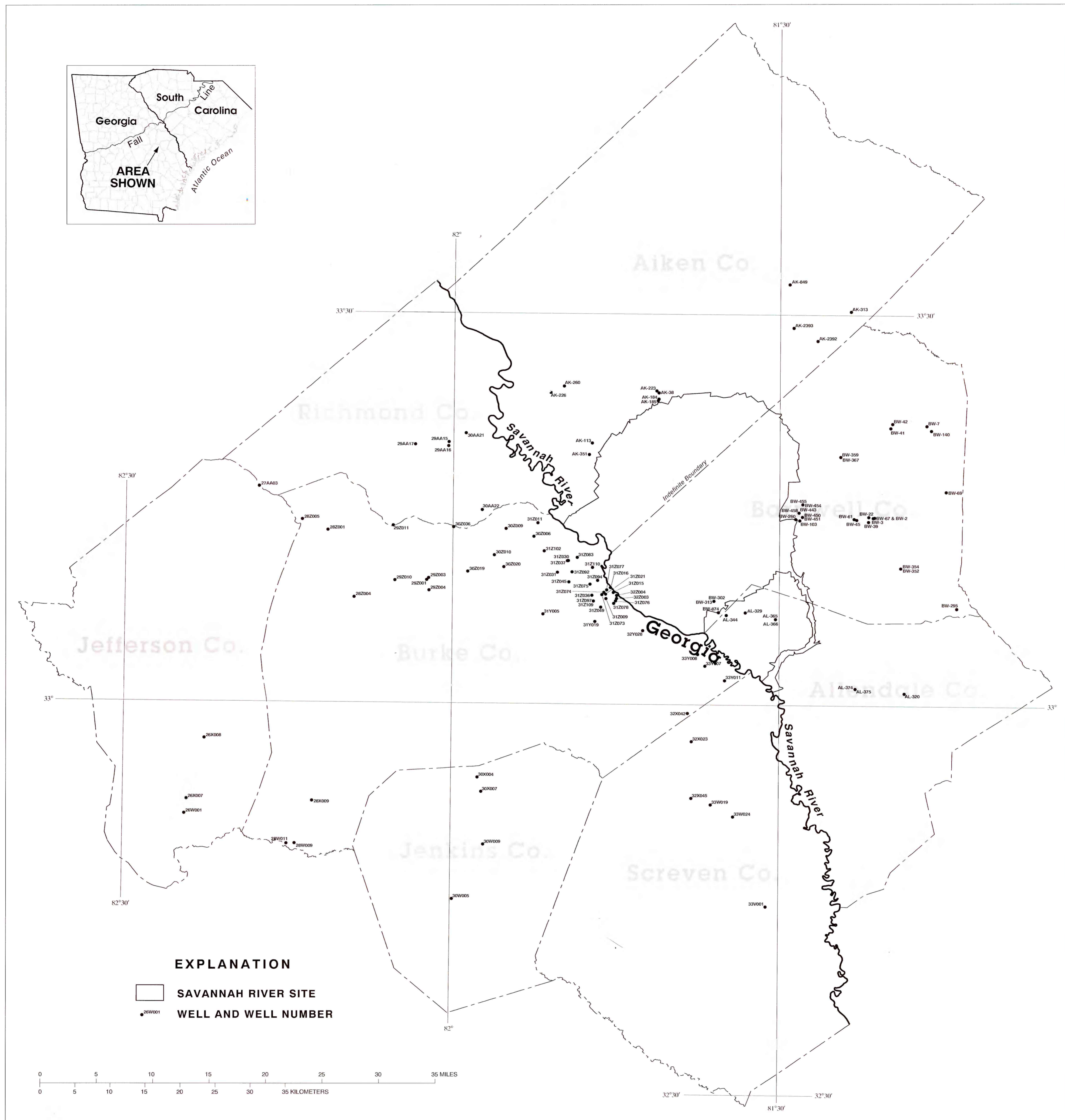
Plate 2. Locations of selected wells for the Gordon aquifer outside the Savannah River Site boundary, South Carolina and Georgia.
