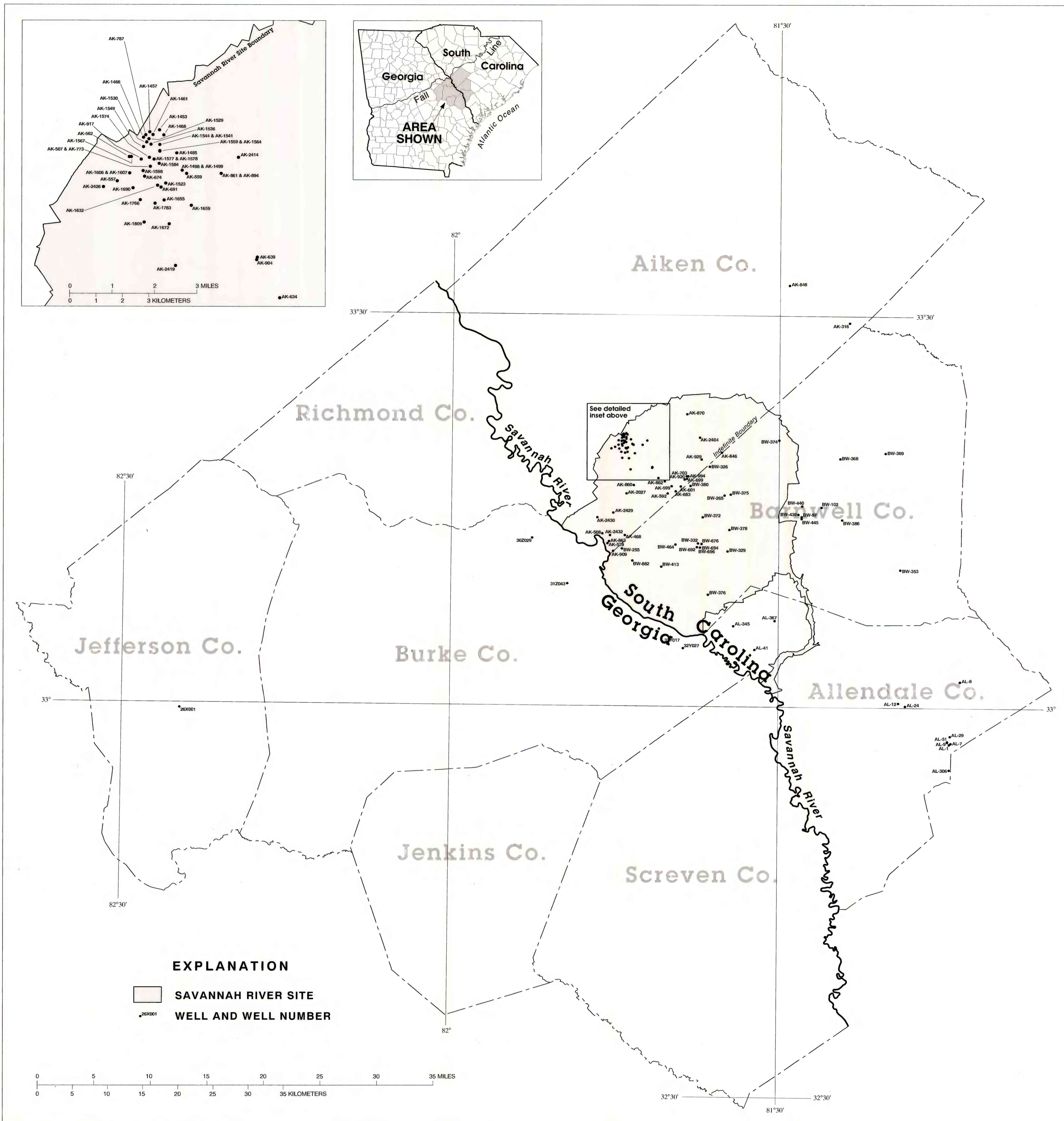
Plate 5. Locations of selected wells for the upper Dublin aquifer, South Carolina and Georgia.
