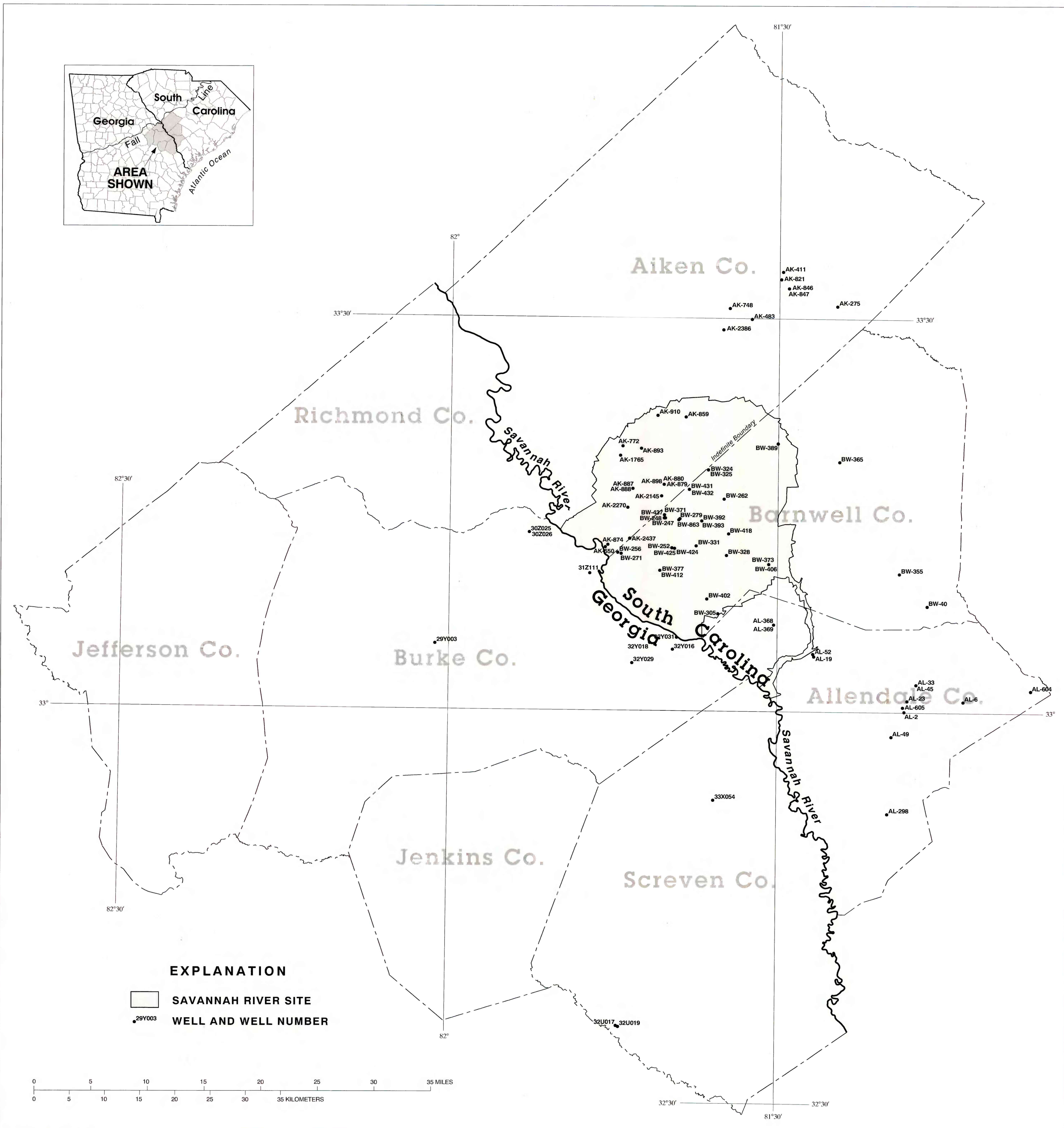
Plate 6. Locations of selected wells for the lower Dublin aquifer, South Carolina and Georgia.
