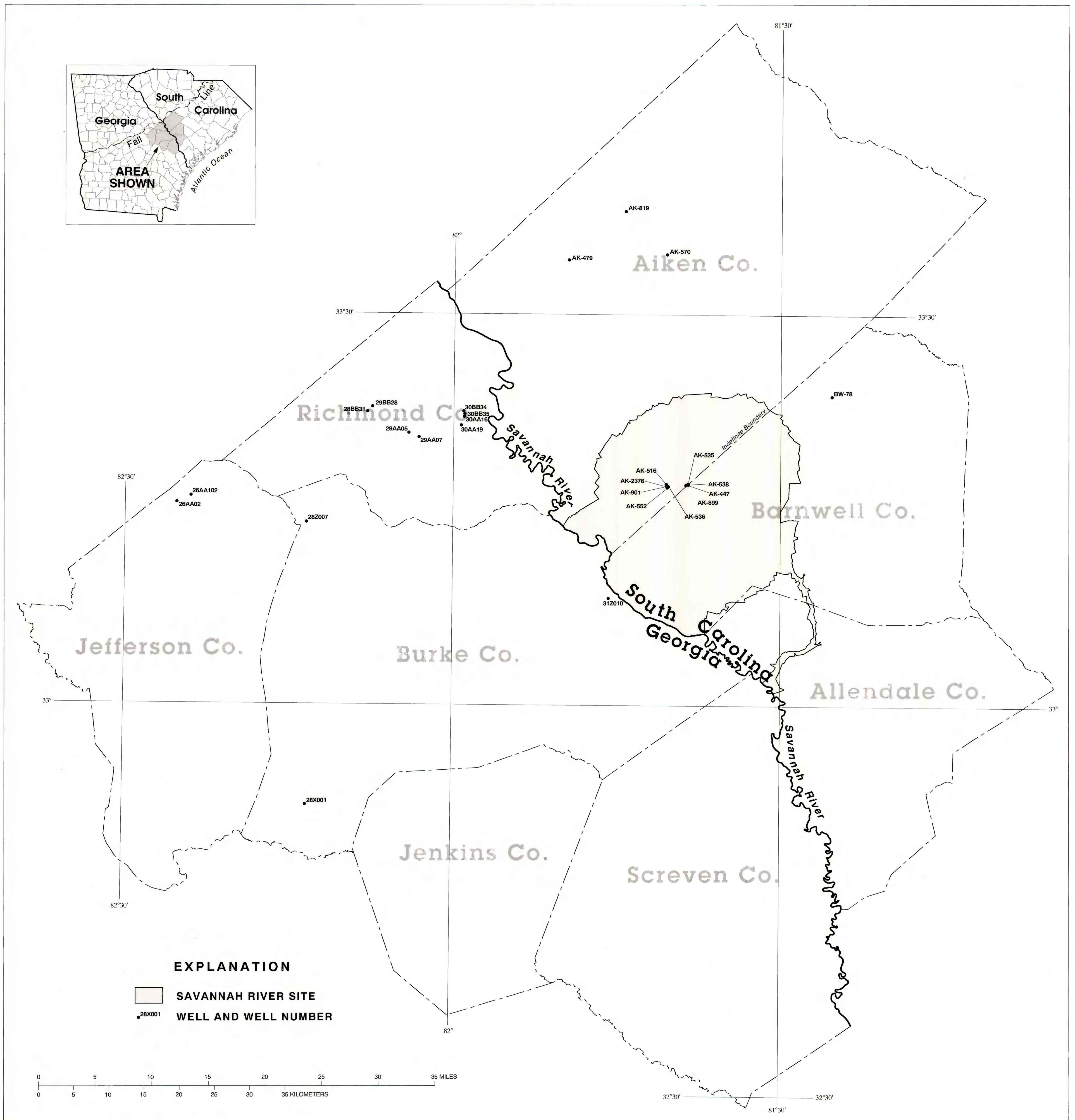
Plate 7. Locations of selected wells for the Midville aquifer system, South Carolina and Georgia.
