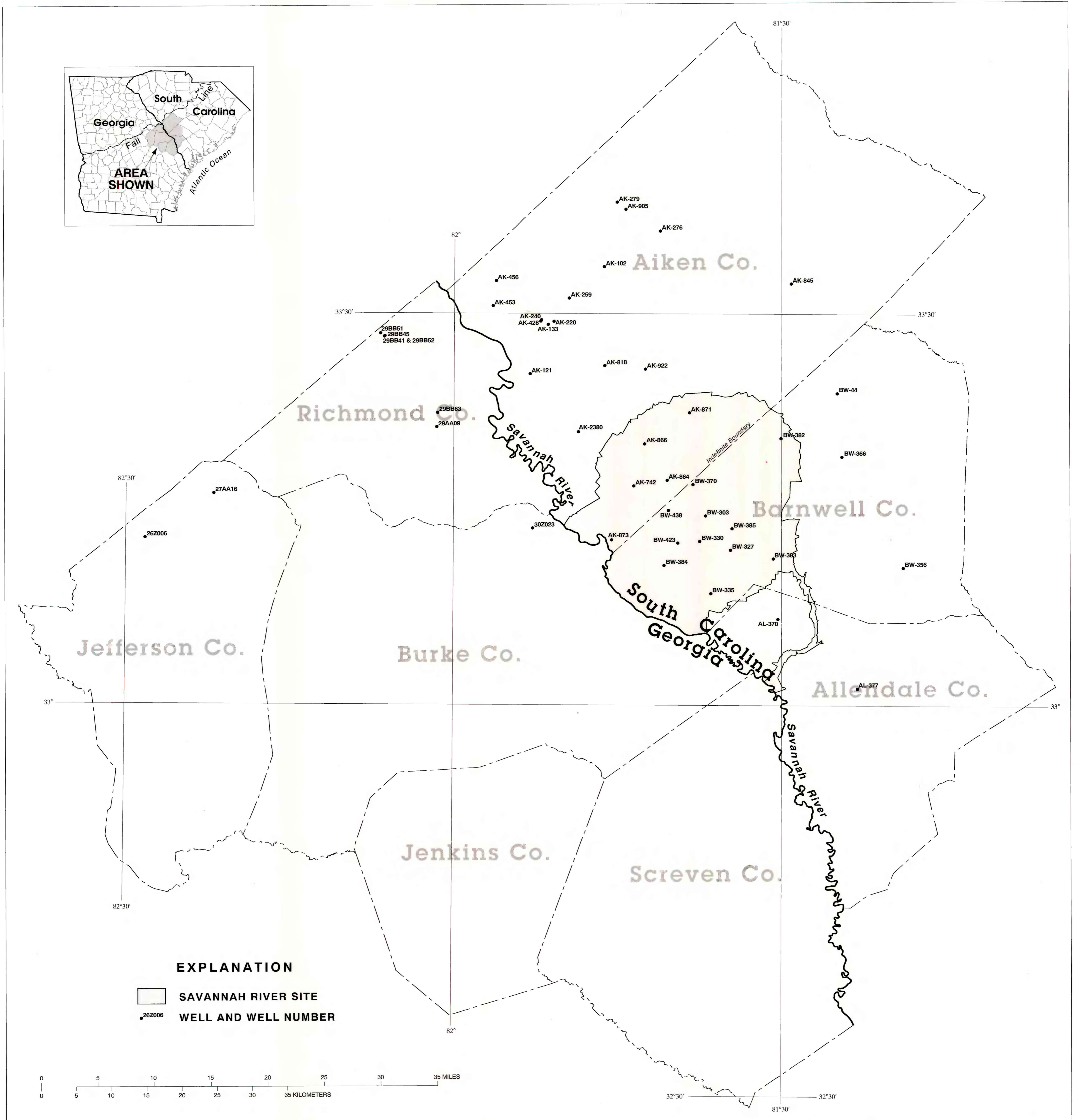
Plate 8. Locations of selected wells for the upper Midville aquifer, South Carolina and Georgia.
