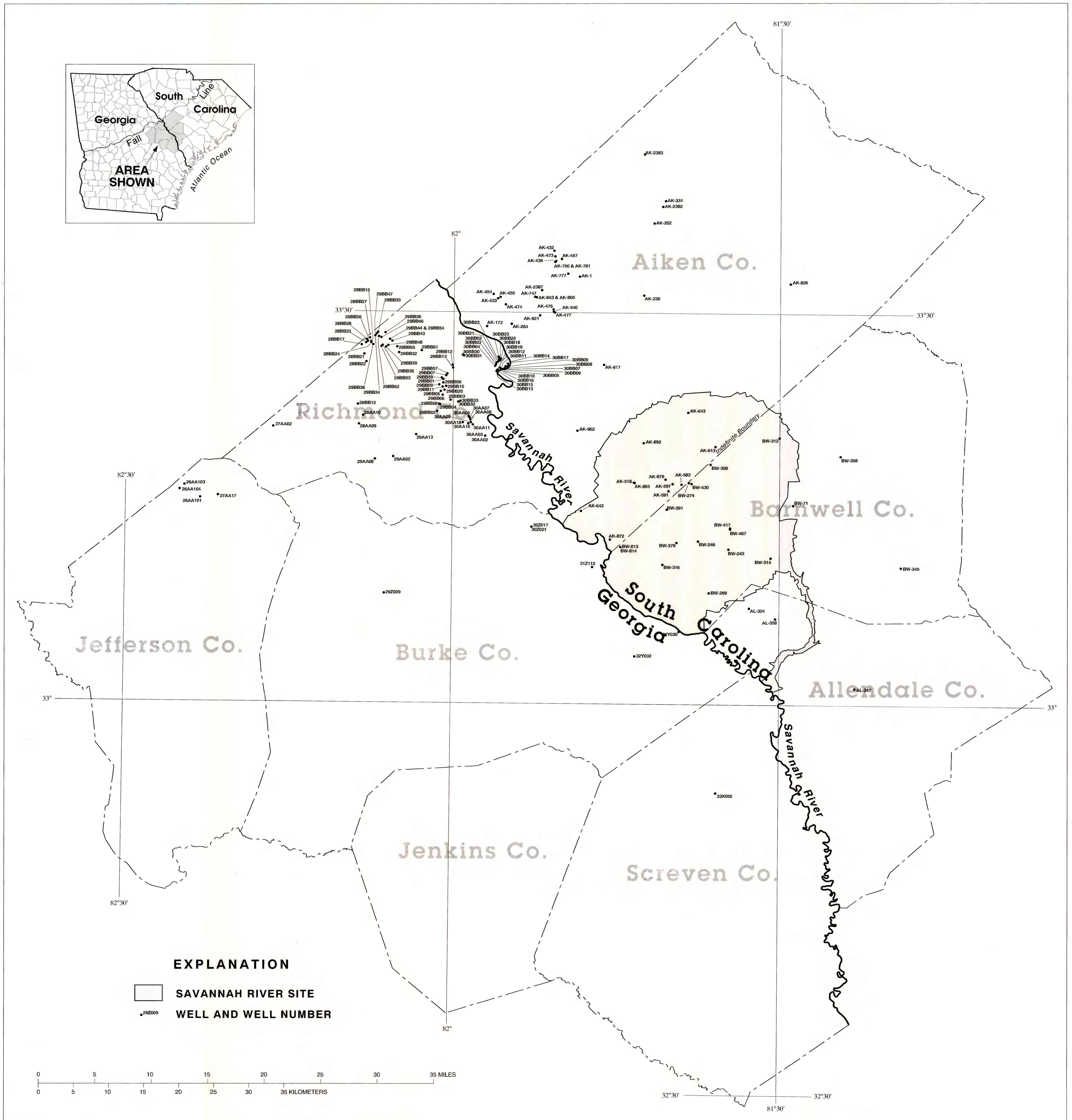
Plate 9. Locations of selected wells for the lower Midville aquifer, South Carolina and Georgia.
