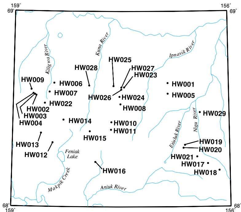
Distribution of mineral occurrences in the Howard Pass 1:250,000-scale quadrangle, north central Alaska
