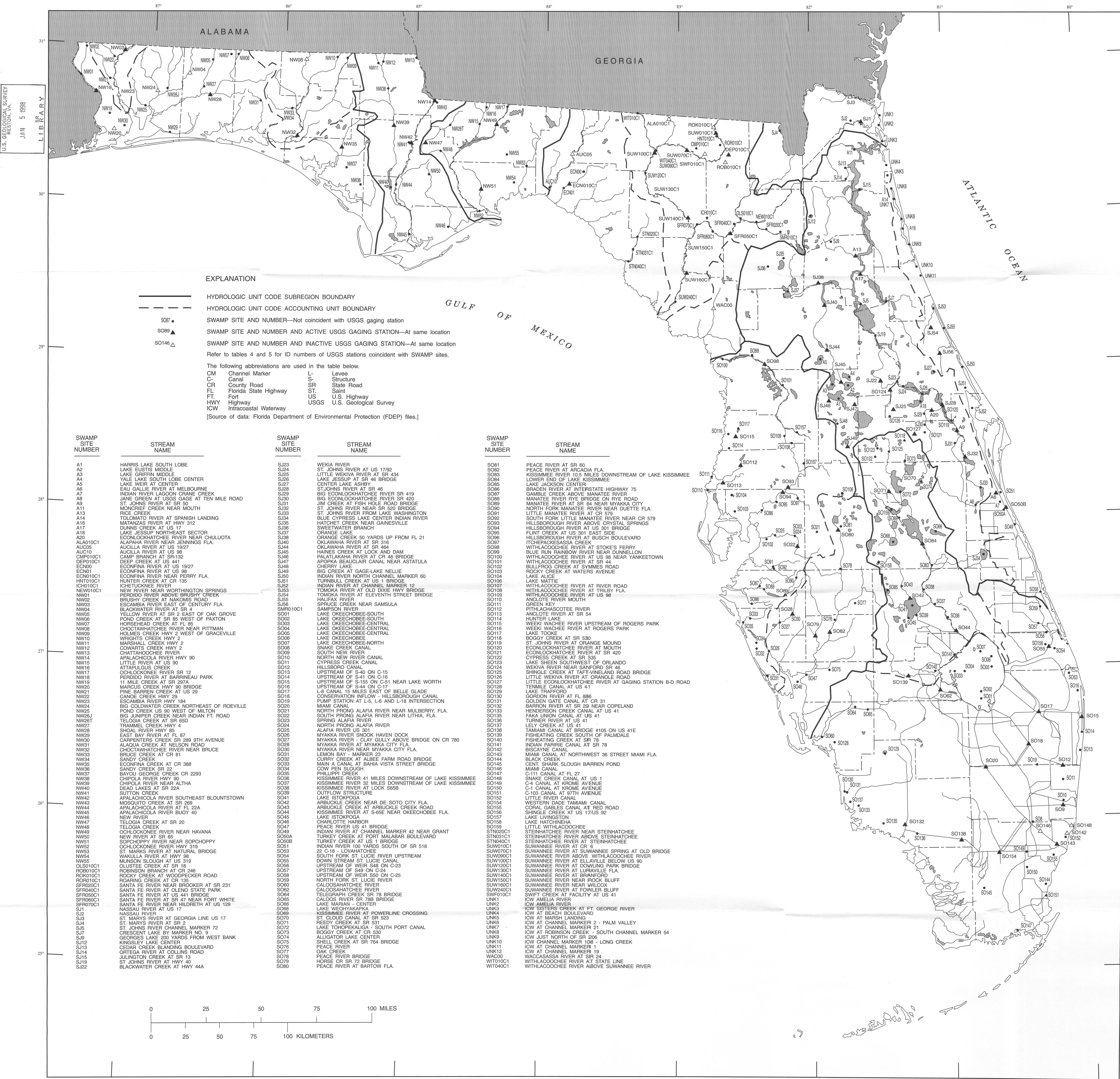
Base map scale 1:1,000,000, digital data source from: U.S. Geological Survey digital data, 1:2,000,000, 1972 Albers Equal-Area Conic projection Standard Parallels 29°30' and 45°30', central meridian 83°00' LOCATIONS OF SWAMP (Surface-Water Ambient Monitoring Program) NETWORK TREND SITES AND COINCIDENT LOCATIONS OF U.S. GEOLOGICAL SURVEY STREAMFLOW-GAGING STATIONS
