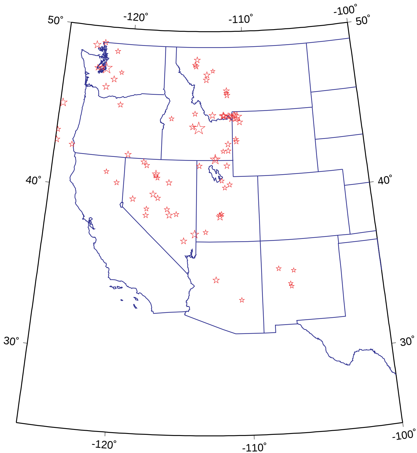
Figure 3b. The USHIS contribution to the WUS catalog during 1964-1985.
