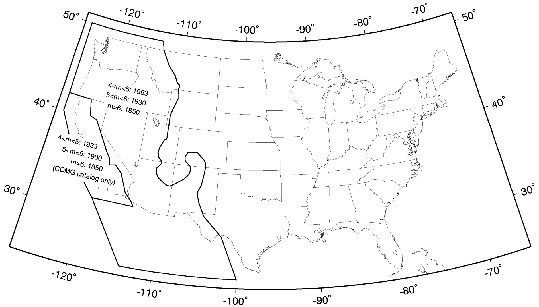
Figure 4. Assumed completeness times for counting earthquakes and computing seismicity rates in WUS.
