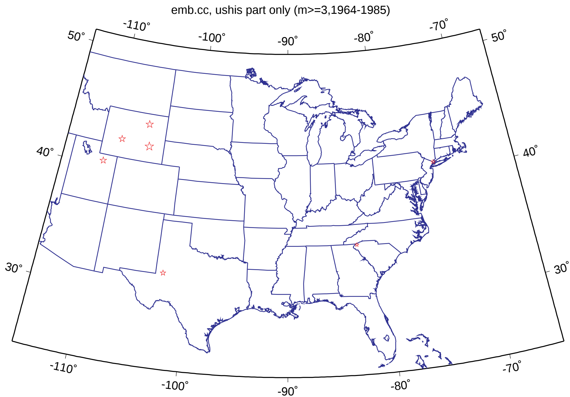
Figure 7c. The USHIS contribution to the CEUS catalog during 1964-1985.
