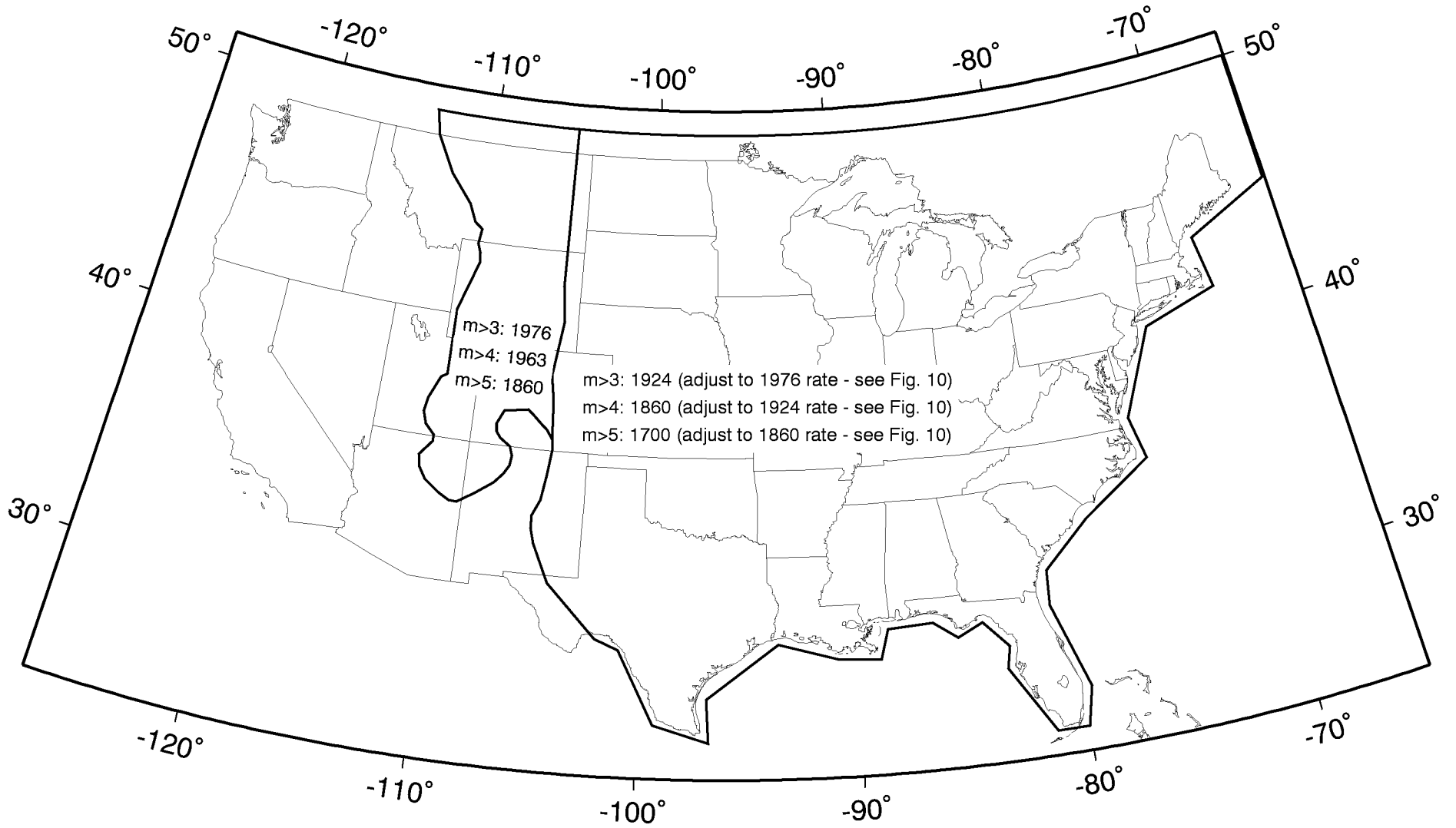
Figure 8. Assumed completeness times for counting earthquakes and computing seismicity rates in CEUS.
