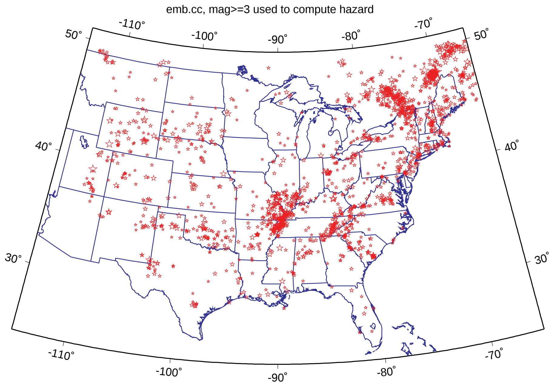
Figure 9a. The CEUS catalog used to compute hazard, magnitude \geq 3 .
