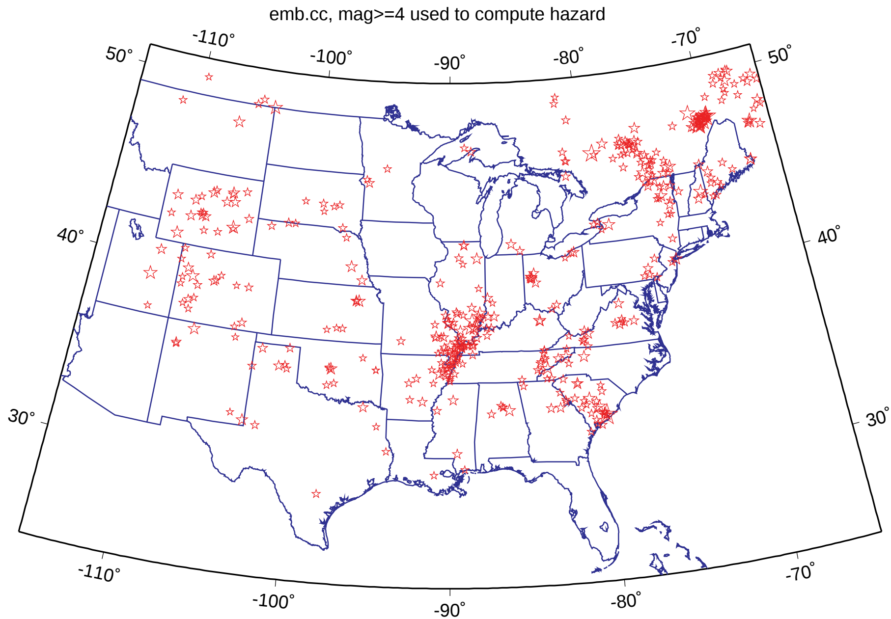
Figure 9b. The CEUS catalog used to compute hazard, magnitude \geq 4 .
