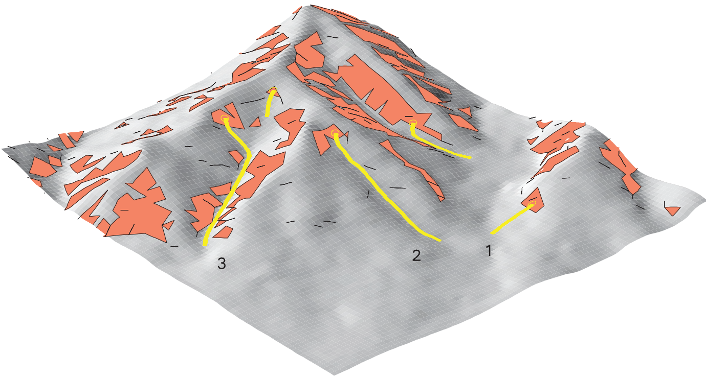
Figure 1: Perspective view showing typical debris flows (yellow) resulting from a major storm, in relation to potential source areas (red zones) like those shown on the map. In any one storm only a small fraction of the potential source areas may be activated. Most debris flows in the San Francisco Bay region travel only several tens of yards or less, but some may travel hundreds of yards downslope from their sources and others have traveled as much as a mile or more down stream channels. Numbers refer to typical hazardous locations discussed above.
