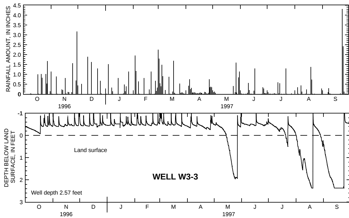
Figure 6. Daily rainfall amounts at wetland and hourly water levels recorded at well W3-3, October 1, 1996 through September 30, 1997.
