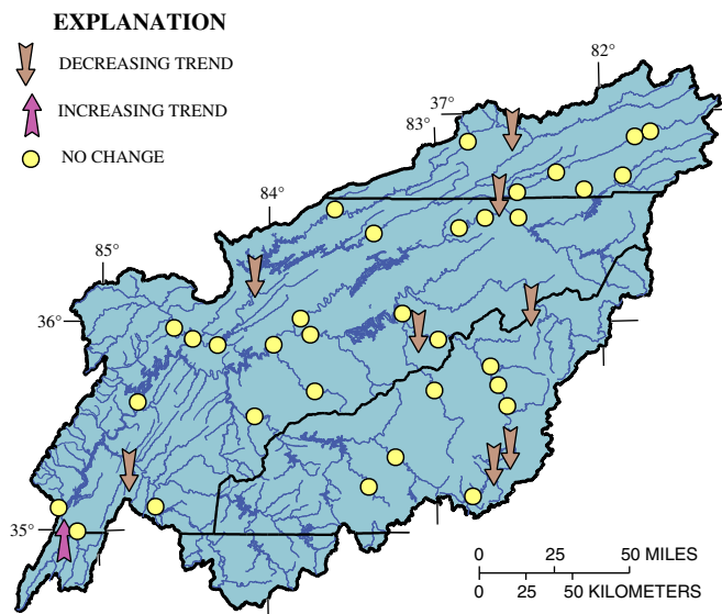
Figure 4. Trends in total phosphorus concentrations, 1970-93.
