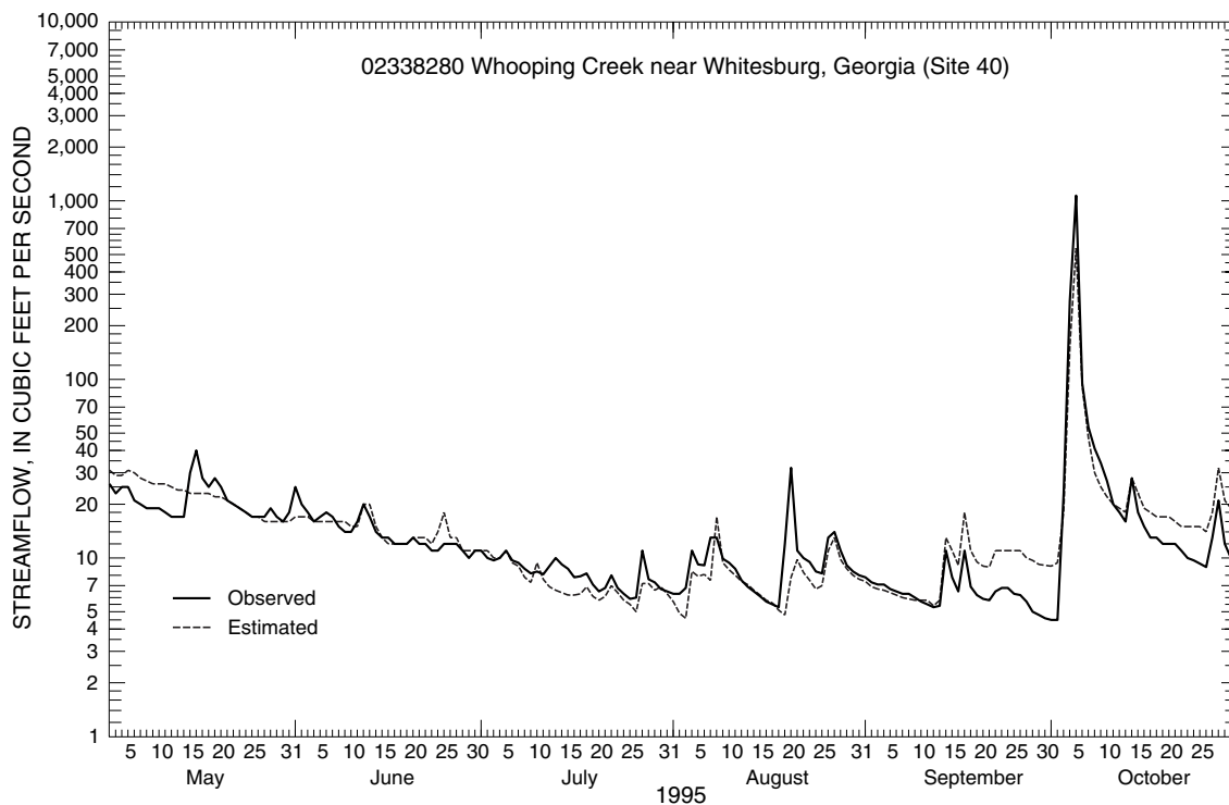
Figure 11. Comparison of observed and estimated daily tributary streamflow data for Whooping Creek near Whitesburg, Georgia.
