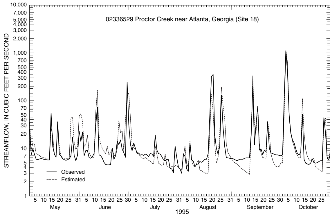
Figure 6. Comparison of observed and estimated daily tributary streamflow data for Proctor Creek near Atlanta, Georgia.
