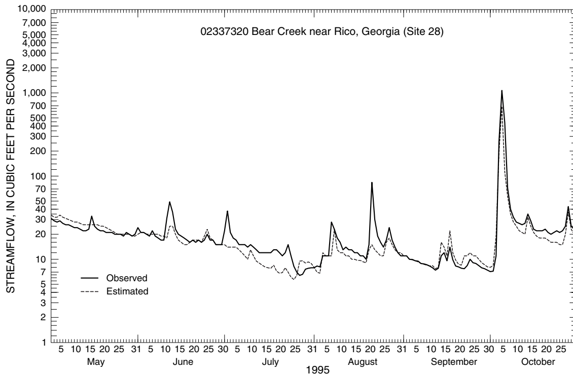
Figure 10. Comparison of observed and estimated daily tributary streamflow data for Bear Creek near Rico, Georgia.
