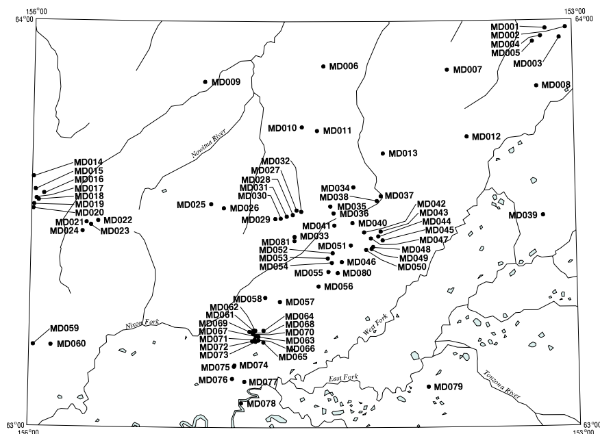
Distribution of mineral occurrences in the Medfra 1:250,000-scale quadrangle, Alaska
