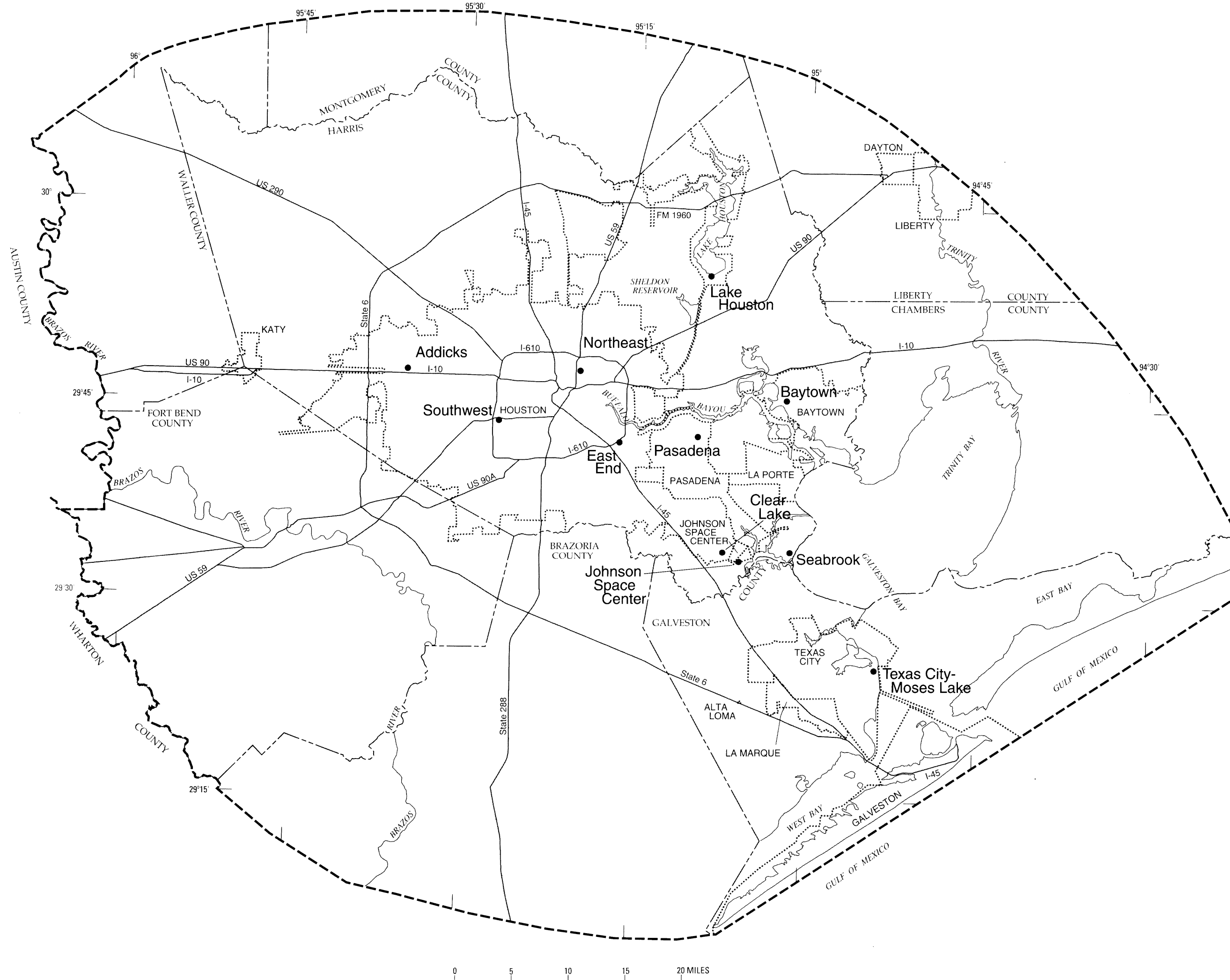
Figure 7. Map showing location of extensometer sites, Houston-Galveston region, Texas.
