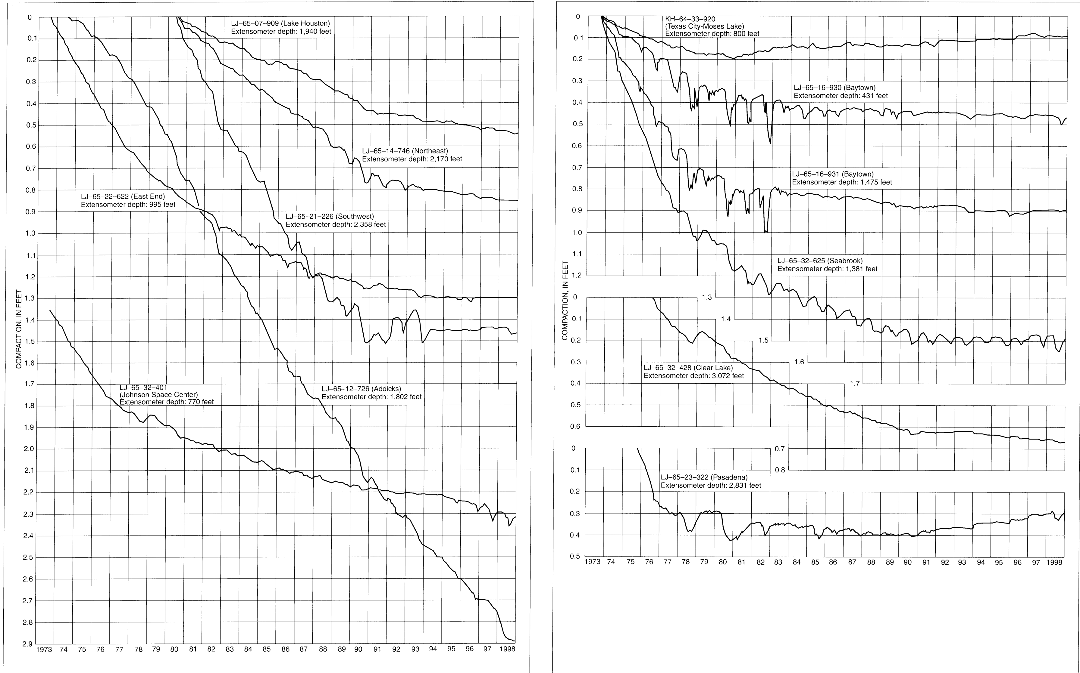
Figure 8. Graphs showing measured compaction of subsurface material, 1973-98, at extensometer sites shown in figure 7.
