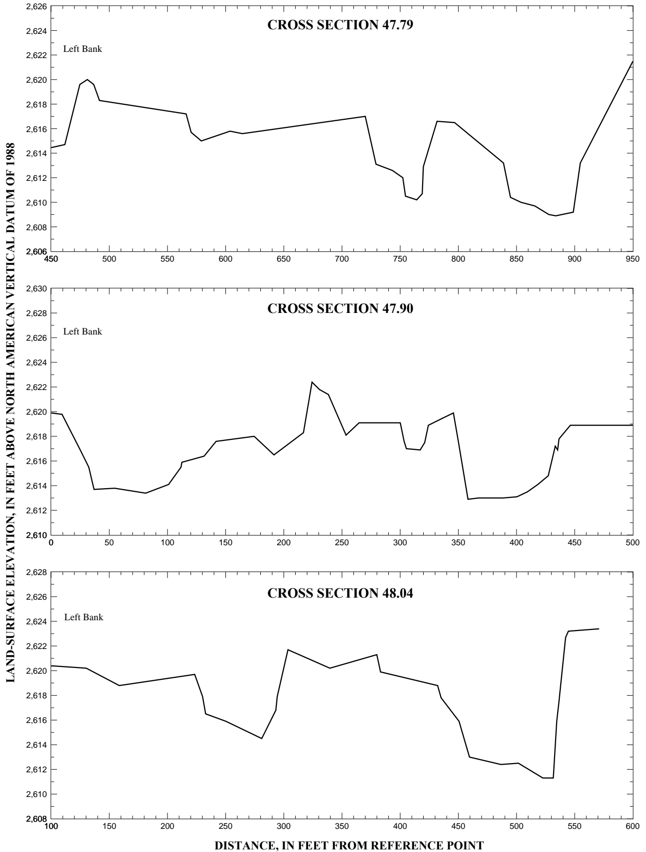
Figure 14. Segments of channel cross sections on the Boise River from river mile 47 to 51, in Ada County, Idaho--Continued.
