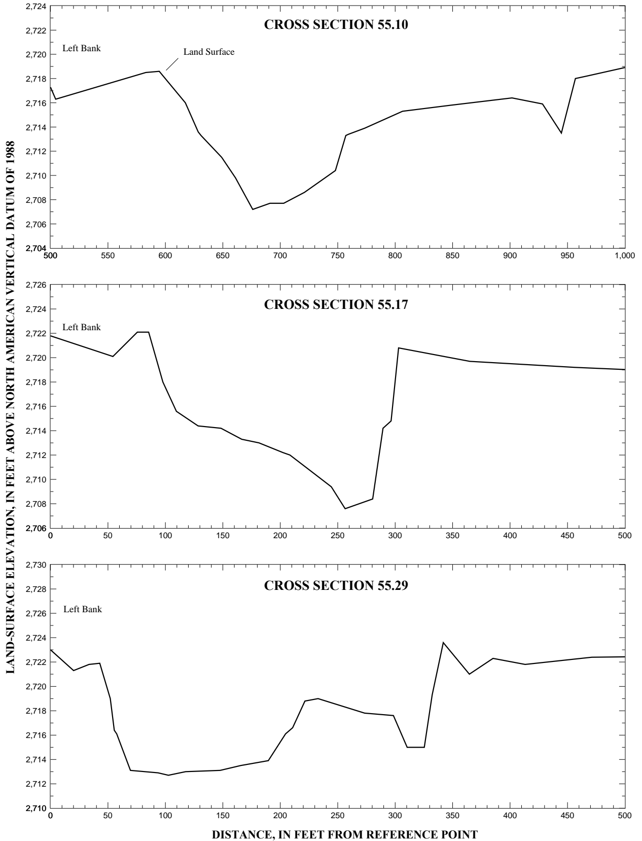
Figure 18. Segments of channel cross sections on the Boise River from river mile 55 to 59, in Ada County, Idaho.
