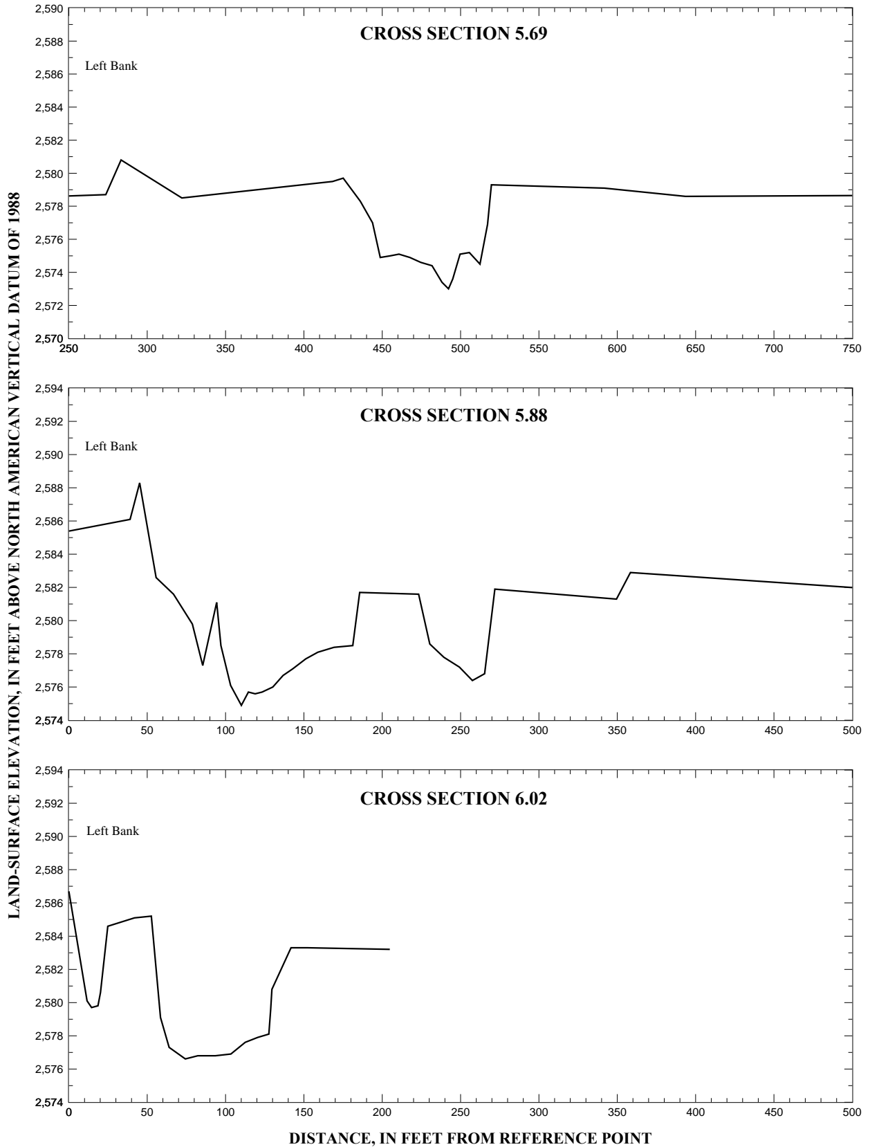
Figure 12. Segments of channel cross sections on the south channel of the Boise River from river mile 3.5 to 6.71, in Ada County, Idaho--Continued.
