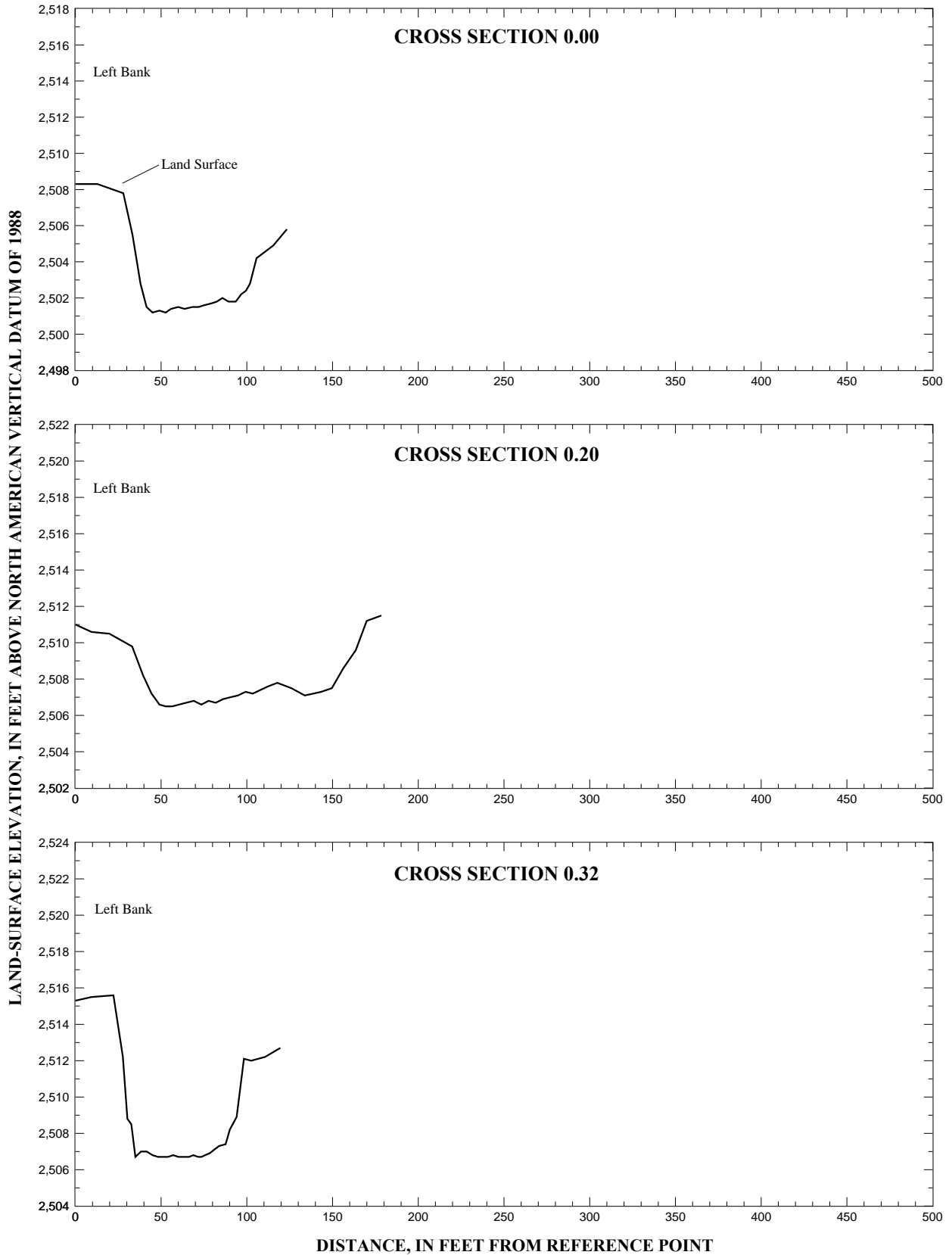
Figure 9. Segments of channel cross sections on the south channel of the Boise River from river mile 0 to 3.5, in Ada County, Idaho.
