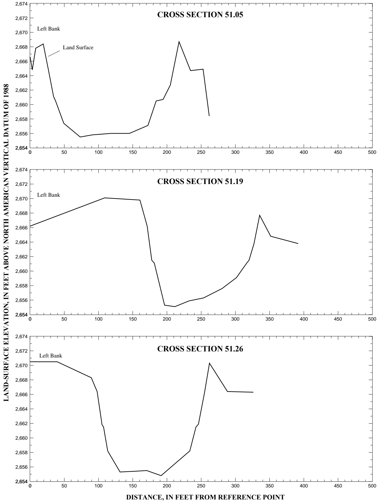
Figure 16. Segments of channel cross sections on the Boise River from river mile 51 to 55, in Ada County, Idaho.
