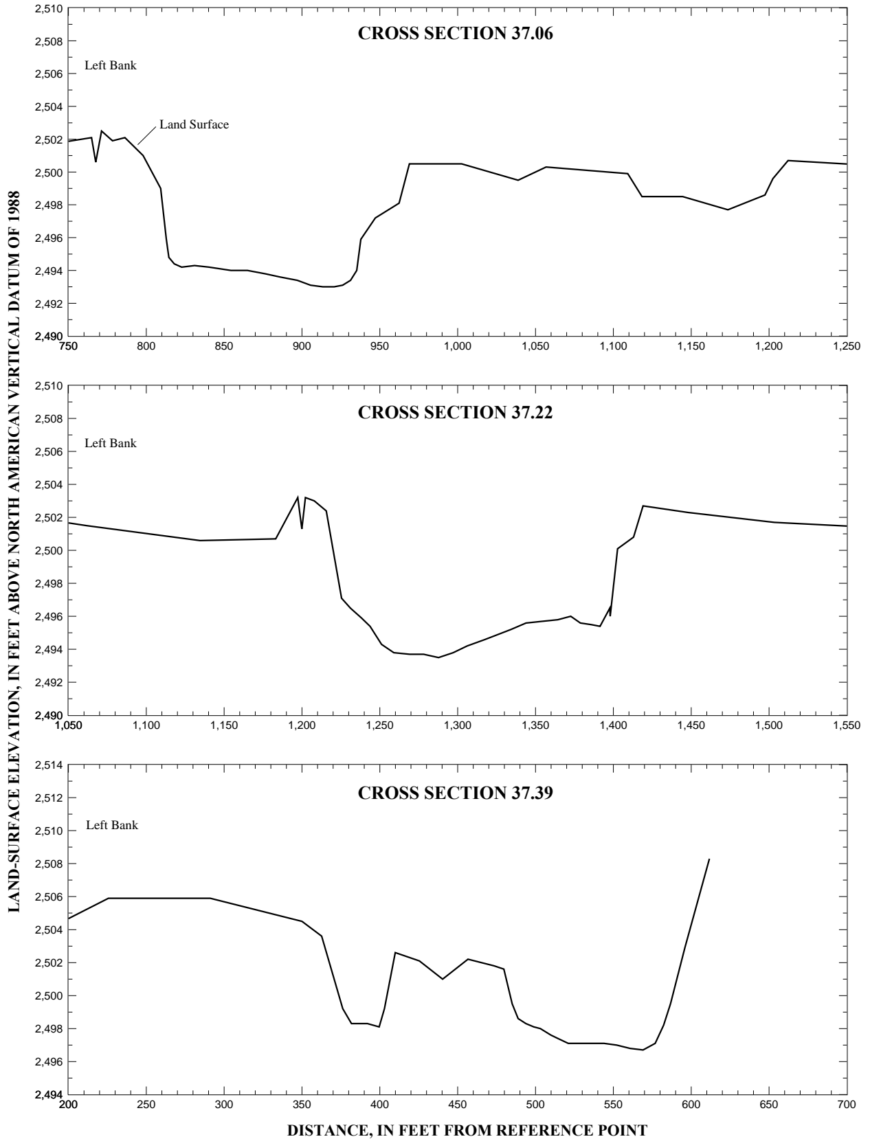
Figure 8. Segments of channel cross sections on the Boise River from river mile 37 to 42, in Ada County, Idaho.
