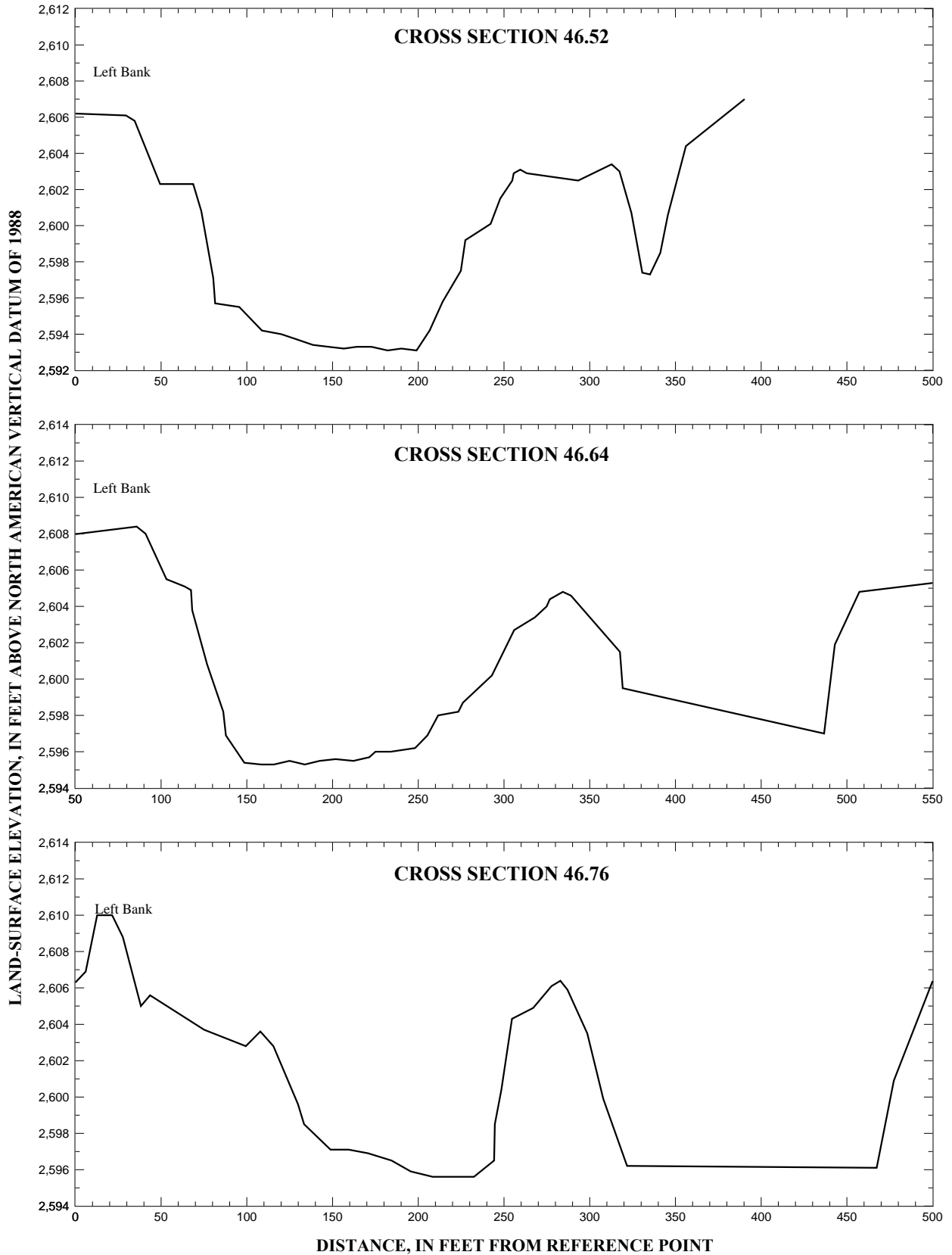
Figure 11. Segments of channel cross sections on the Boise River from river mile 42 to 47, in Ada County, Idaho--Continued.
