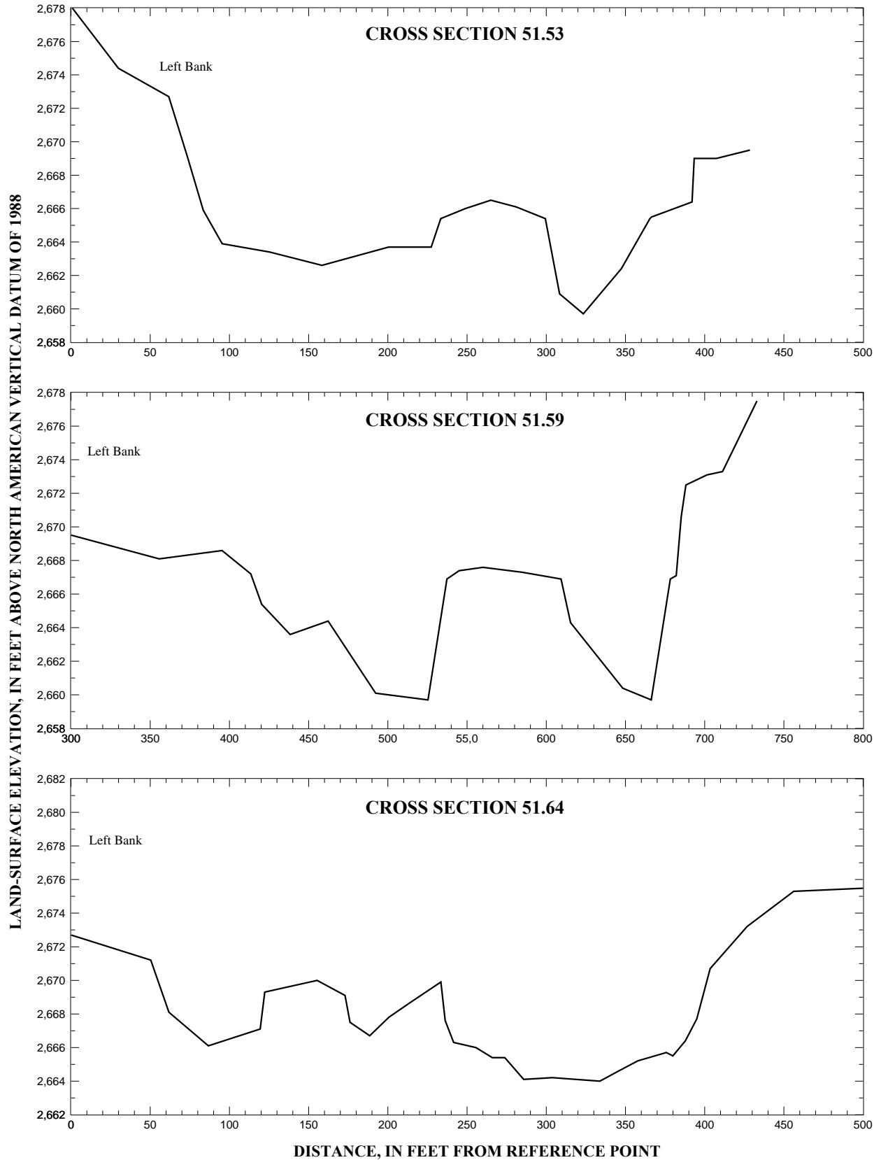
Figure 16. Segments of channel cross sections on the Boise River from river mile 51 to 55, in Ada County, Idaho--Continued.
