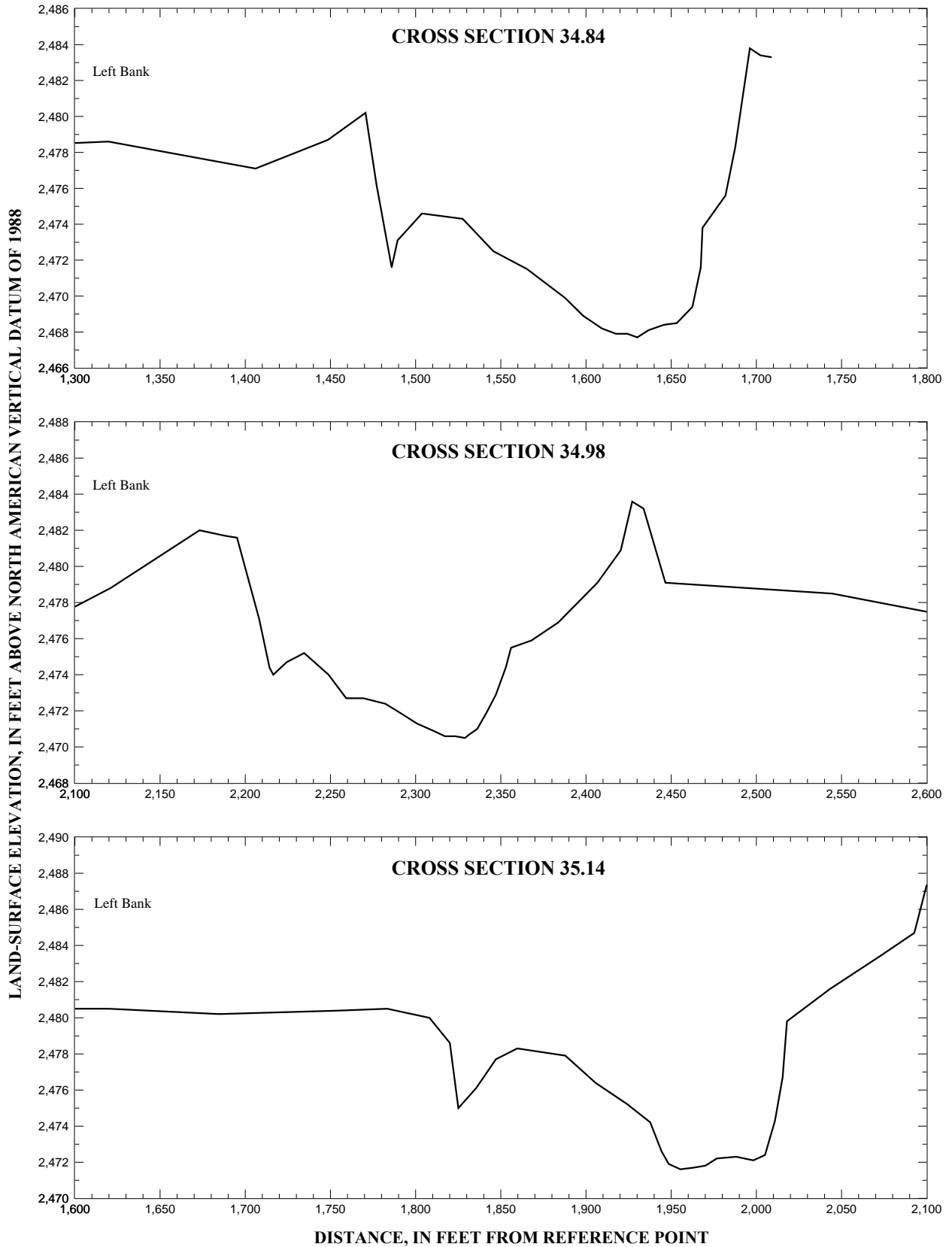
Figure 6. Segments of channel cross sections on the Boise River from the Ada/Canyon County boundary to river mile 37, in Ada County, Idaho--Continued.
