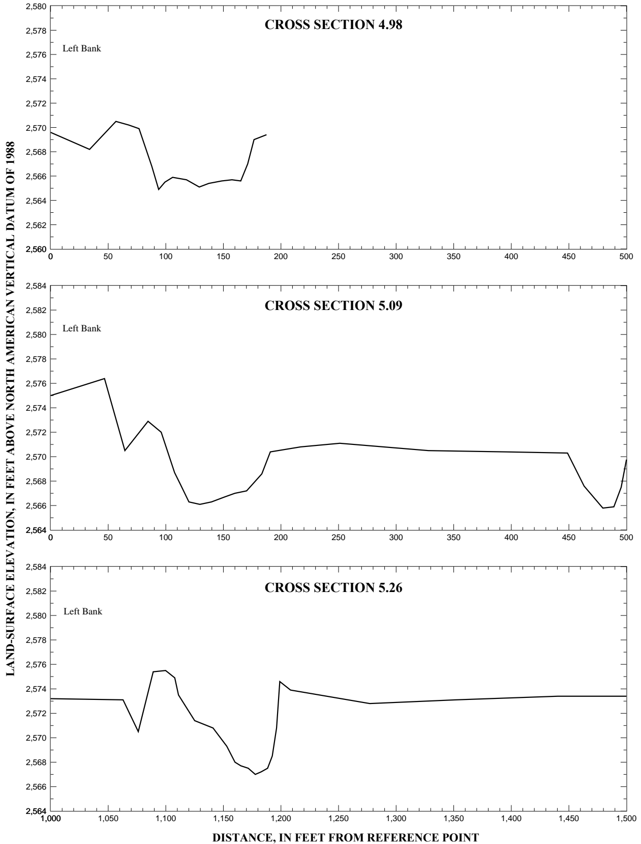
Figure 12. Segments of channel cross sections on the south channel of the Boise River from river mile 3.5 to 6.71, in Ada County, Idaho--Continued.
