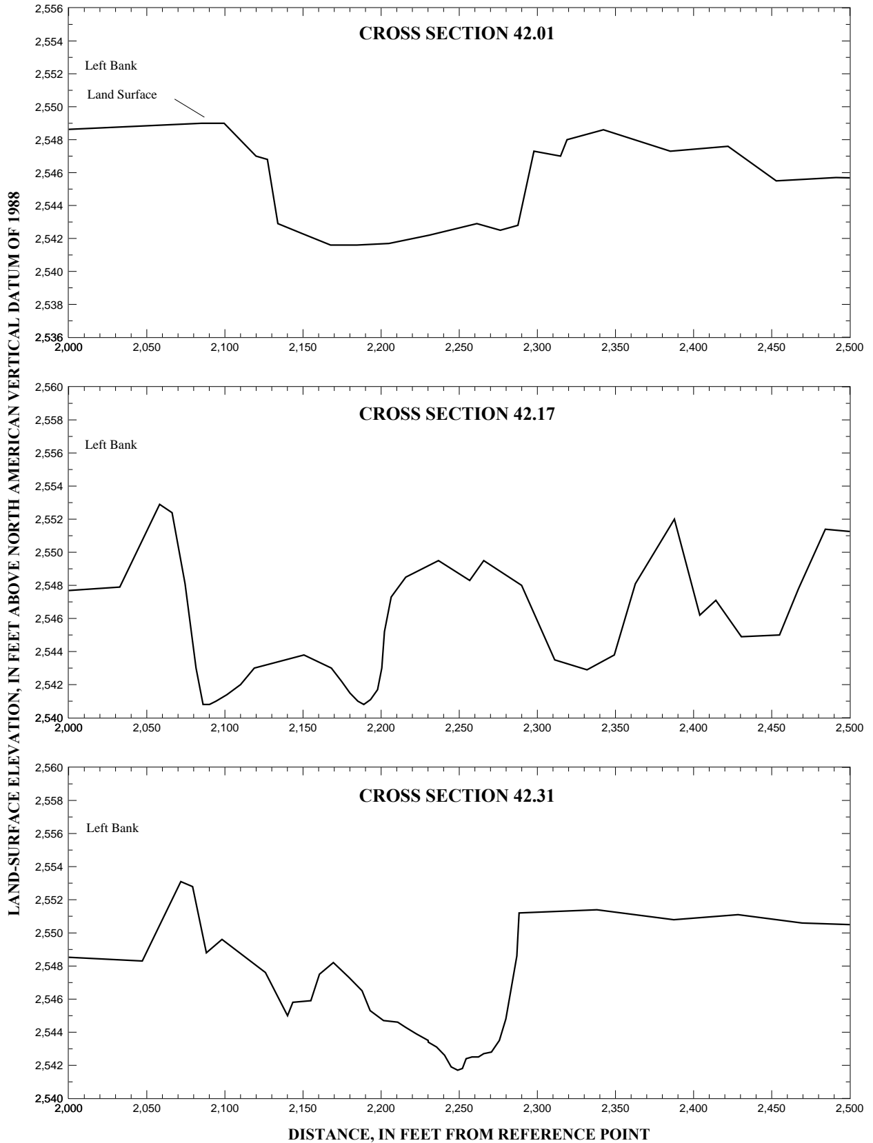
Figure 11. Segments of channel cross sections on the Boise River from river mile 42 to 47, in Ada County, Idaho.
