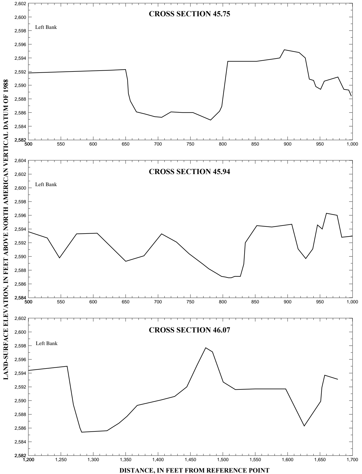
Figure 11. Segments of channel cross sections on the Boise River from river mile 42 to 47, in Ada County, Idaho--Continued.
