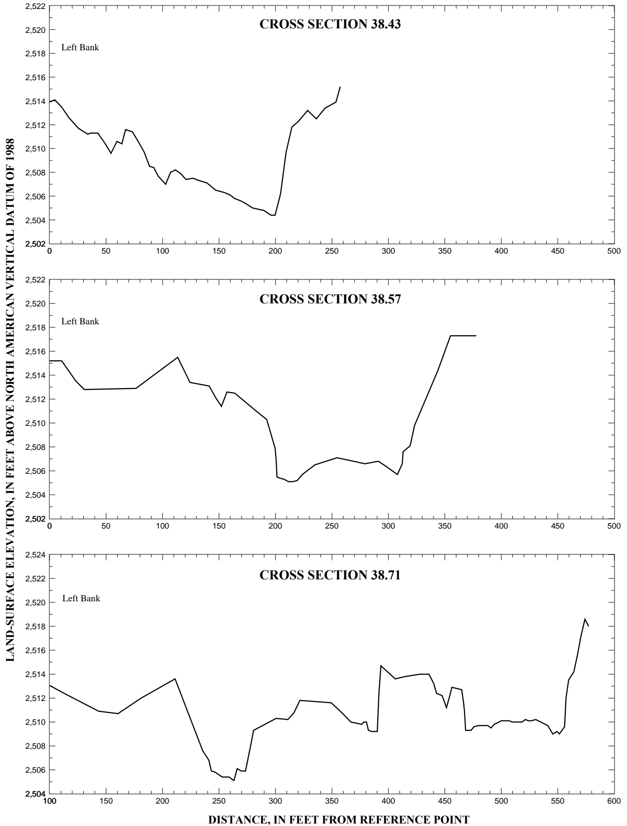
Figure 8. Segments of channel cross sections on the Boise River from river mile 37 to 42 in Ada County, Idaho--Continued.
