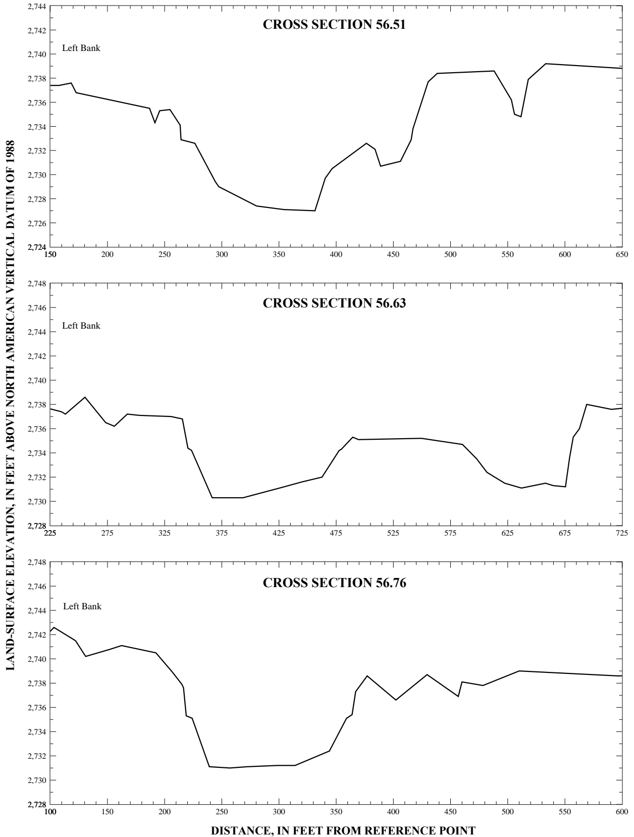
Figure 18. Segments of channel cross sections on the Boise River from river mile 55 to 59, in Ada County, Idaho--Continued.
