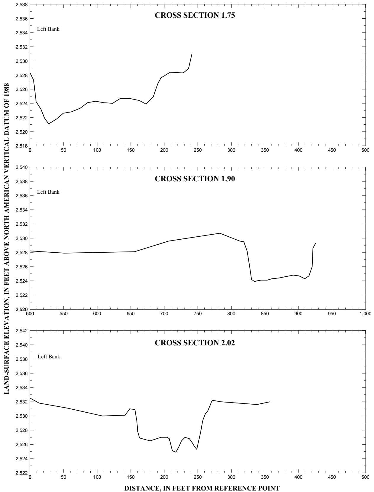
Figure 9. Segments of channel cross sections on the south channel of the Boise River from river mile 0 to 3.5, in Ada County, Idaho--Continued.
