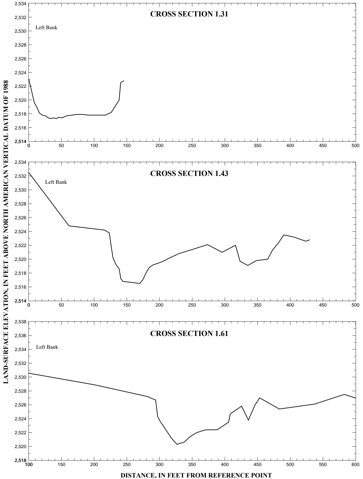
Figure 9. Segments of channel cross sections on the south channel of the Boise River from river mile 0 to 3.5, in Ada County, Idaho--Continued.
