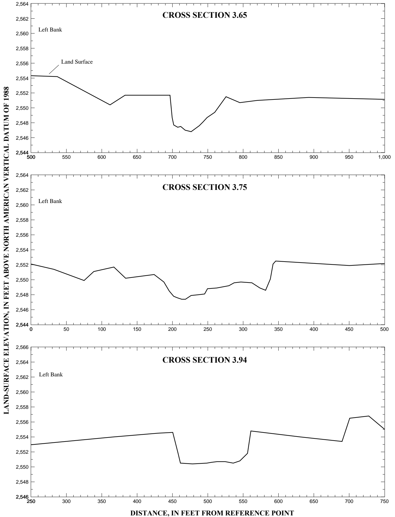
Figure 12. Segments of channel cross sections on the south channel of the Boise River from river mile 3.5 to 6.71, in Ada County, Idaho.
