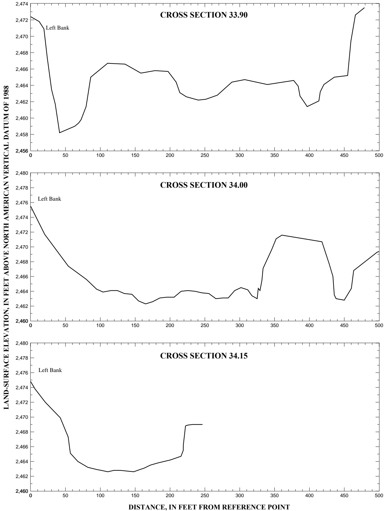
Figure 6. Segments of channel cross sections on the Boise River from the Ada/Canyon County boundary to river mile 37, in Ada County, Idaho--Continued.
