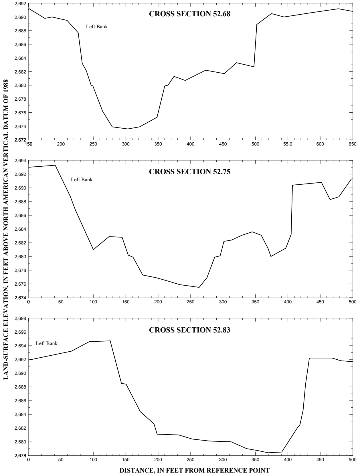
Figure 16. Segments of channel cross sections on the Boise River from river mile 51 to 55, in Ada County, Idaho--Continued.
