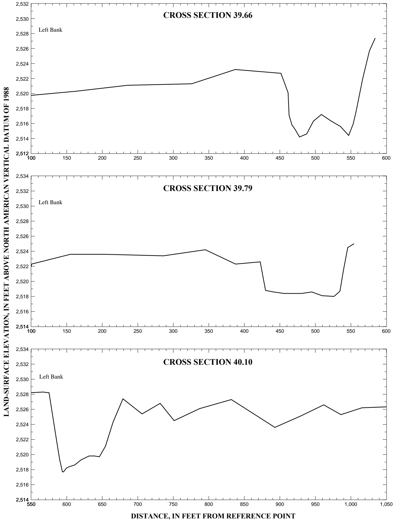
Figure 8. Segments of channel cross sections on the Boise River from river mile 37 to 42 in Ada County, Idaho--Continued.
