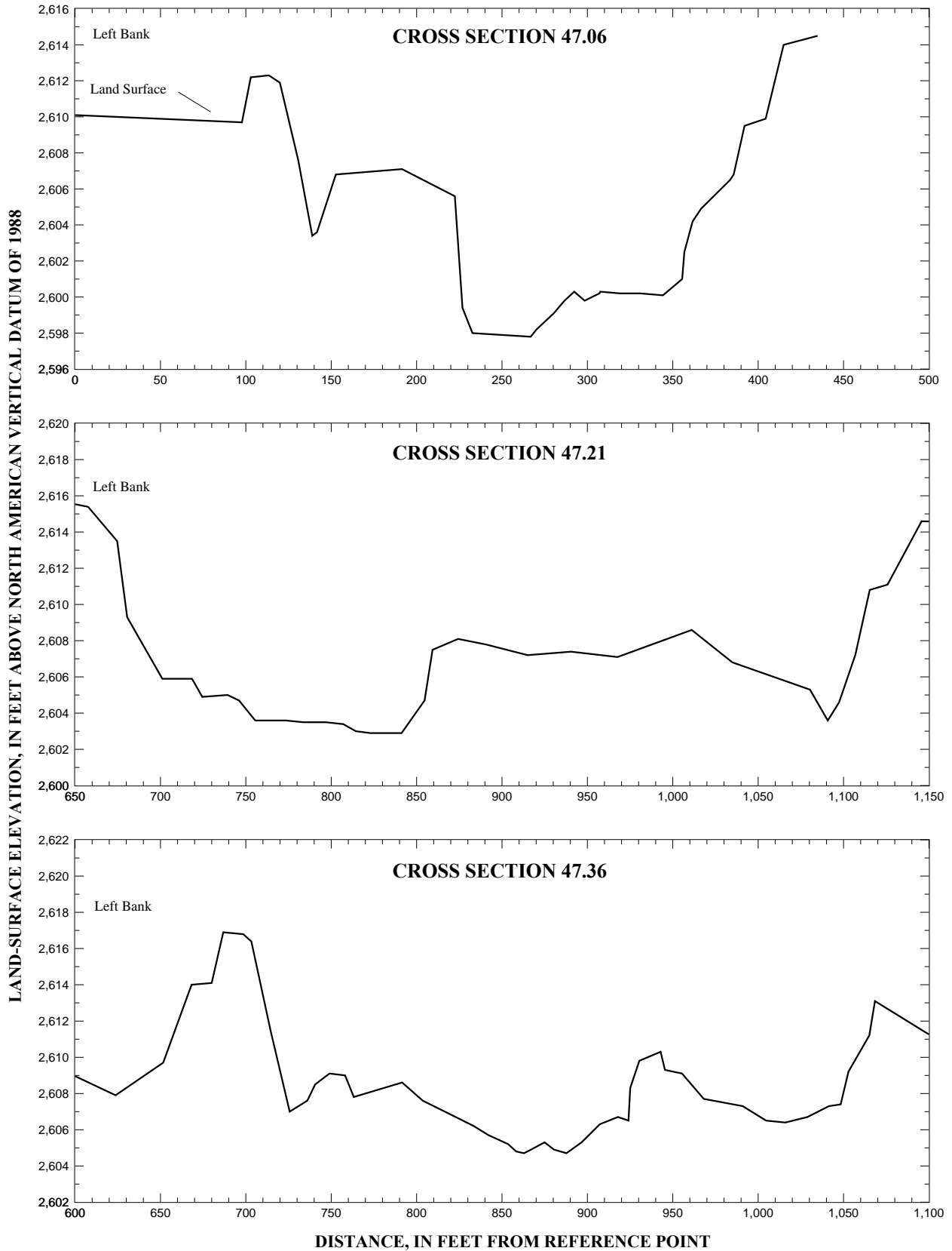
Figure 14. Segments of channel cross sections on the Boise River from river mile 47 to 51, in Ada County, Idaho.
