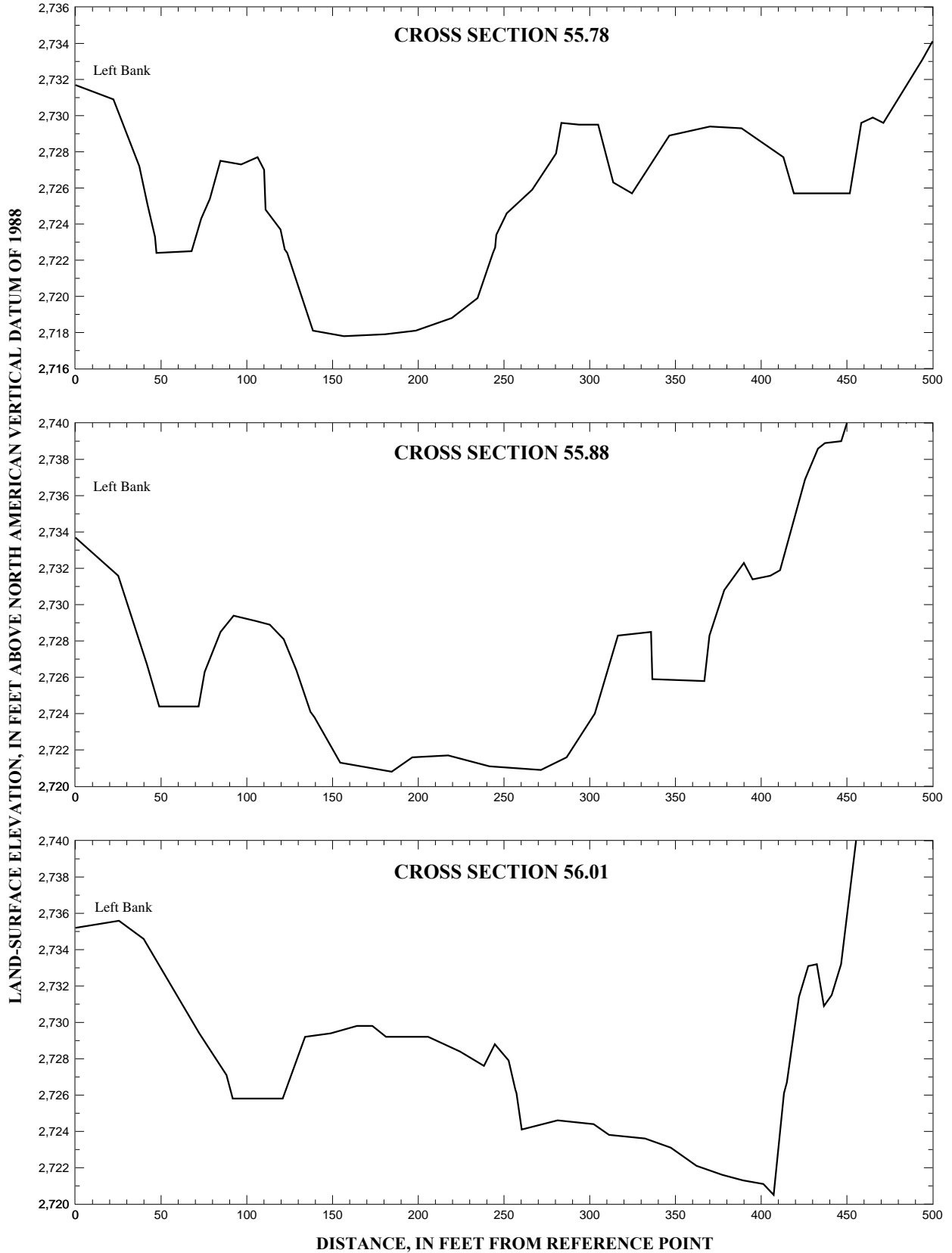
Figure 18. Segments of channel cross sections on the Boise River from river mile 55 to 59, in Ada County, Idaho--Continued.
