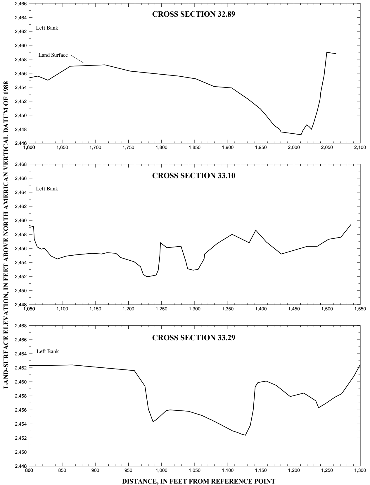
Figure 6. Segments of channel cross sections on the Boise River from the Ada/Canyon County boundary to river mile 37, in Ada County, Idaho.
