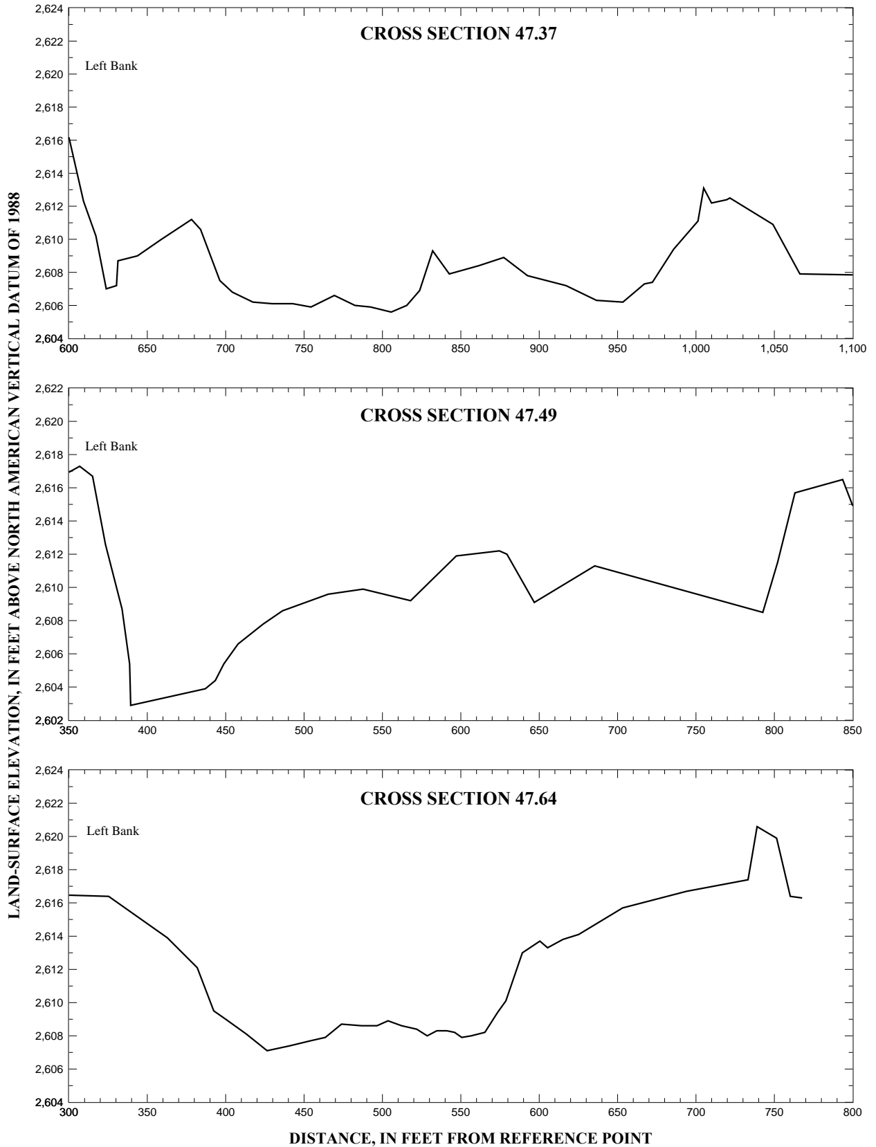
Figure 14. Segments of channel cross sections on the Boise River from river mile 47 to 51, in Ada County, Idaho--Continued.
