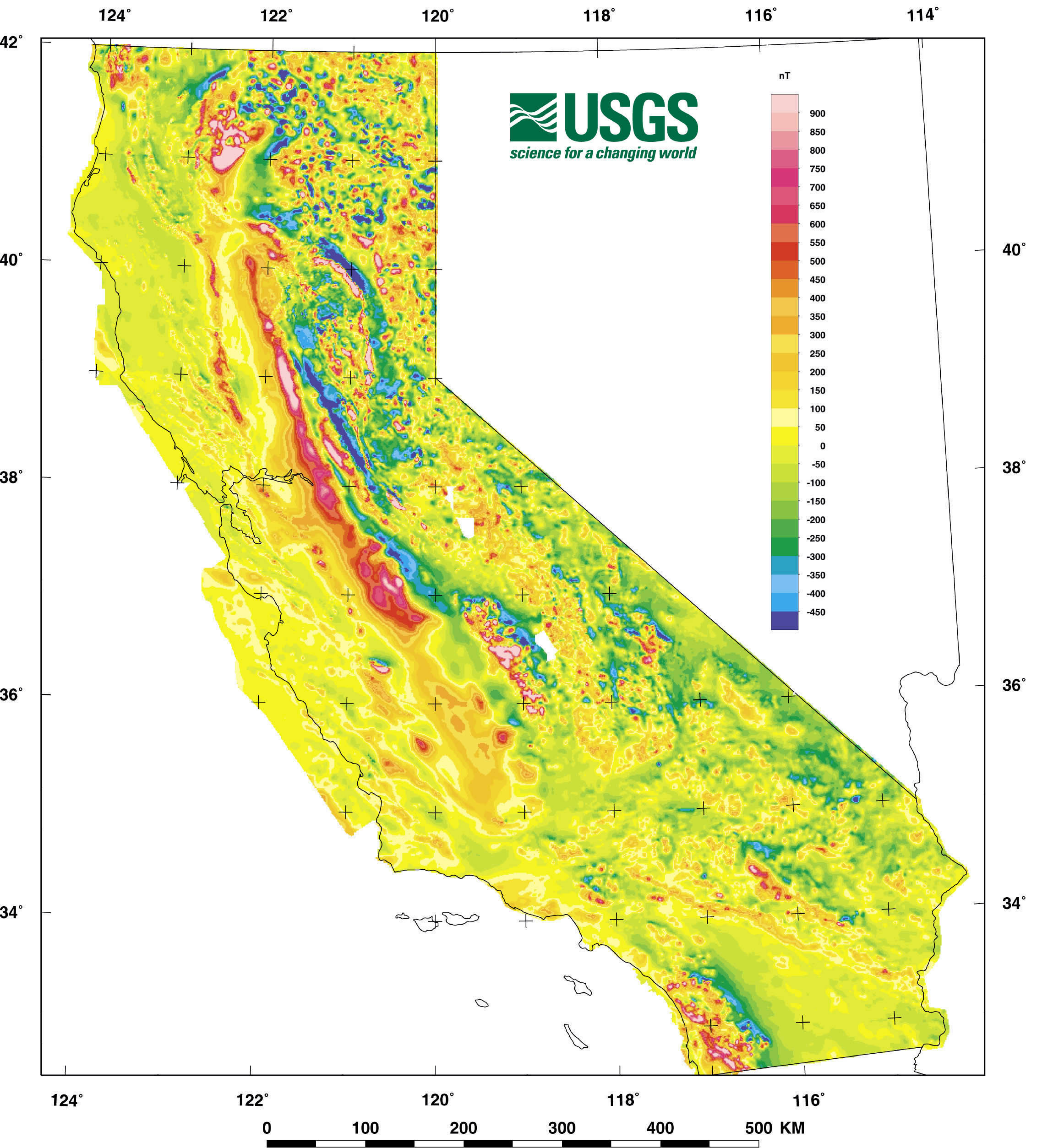
Figure 2. Preliminary aeromagnetic anomaly map of California.
